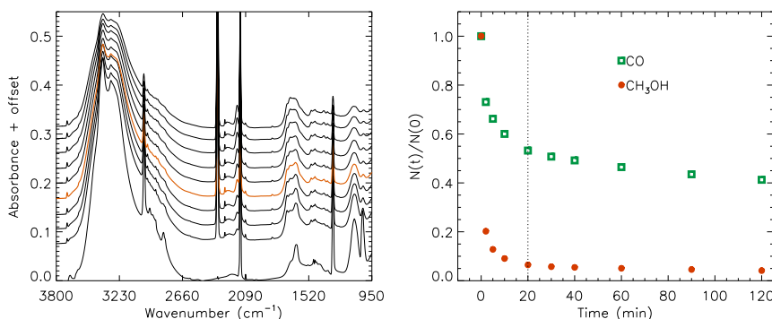
Fig. 1. ( Left ) Infrared spectra of the bilayer ice before irradiation (bottom curve) and after each irradiation step. The orange spectrum is obtained after the fourth irradiation step. The spectra have been shifted for clarity. ( Right ) Column densities of CO and \text{CH}_3\text{OH} normalized to their initial values as functions of the irradiation time. The vertical dotted line marks the fourth irradiation step.
