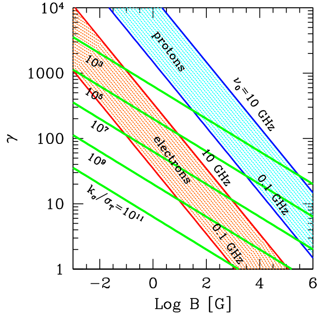
Figure 2. The two general constraints to have efficient synchrotron masers are illustrated in the plane \gamma – B . The (green) lines corresponds to different values of k_\sigma (equation 13), while the two hatched regions corresponds to have the frequencies, at which the cross-section turns negative, in the gigahertz band (equation 12). The hatched region on the left is for electrons, the one on the right is for protons (as labelled). We assume t = 10 and \theta = \pi/2 .
