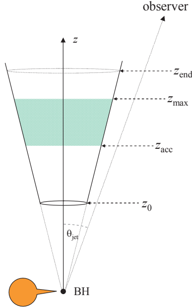
Fig. 1 Detail of a generic conical jet model, including the acceleration region (not to scale). Some relevant parameters are indicated.
