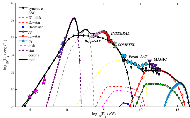
Fig. 13 Spectral energy distribution of the jet of the galactic microquasar Cygnus X-1. From Pepe et al. (2015).
