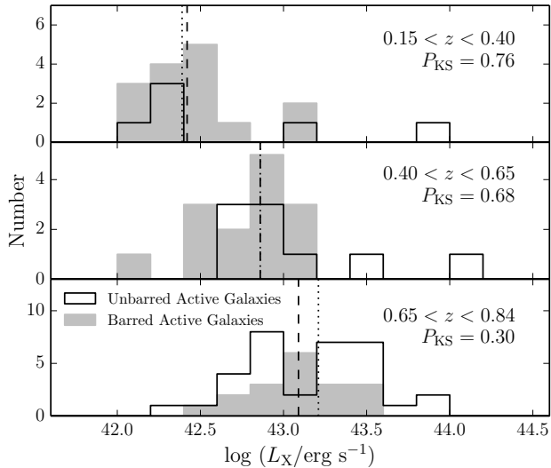
Figure 6. X-ray luminosity distributions of barred (gray histograms) and unbarred (empty histograms) active galaxies over three redshift intervals, with their corresponding p -value from K-S test, P_{\text{KS}} . For each distribution, we show its median as vertical dashed (barred) and dotted (unbarred) lines.
