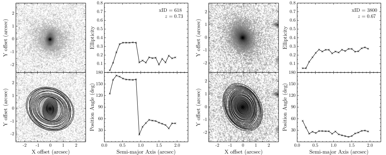
Figure 1. Example results from the ellipse fitting task for a barred active galaxy at z = 0.73 (left panels), and for an unbarred active galaxy at z = 0.67 corresponding to the X-ray sources xID=618 and xID=3800 respectively (Civano et al. 2012). For each galaxy, we show the HST /ACS F814W cutout (top-left), as well as the galaxy isophotes overlaid (bottom-left). For the barred galaxy, its ellipticity profile (top-right) shows a steep drop at 0''.9 , which is matched by a sharp change in its position angle profile (bottom-right) at the same semi-major axis distance, in contrast with the rather smooth profiles of the unbarred galaxy.
