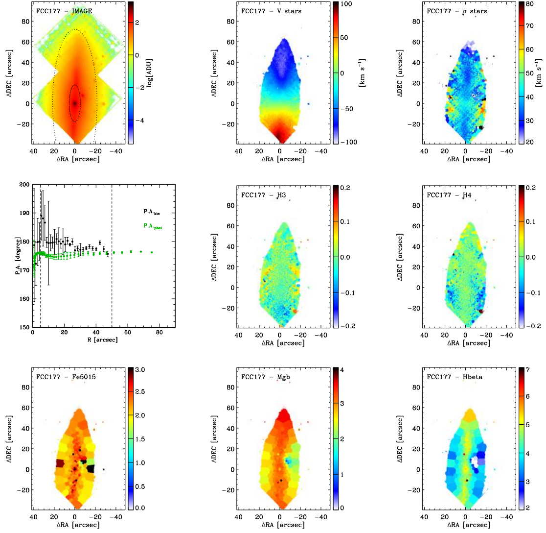
Fig. A.13. Same as in Fig. A.1, but for FCC 177.
