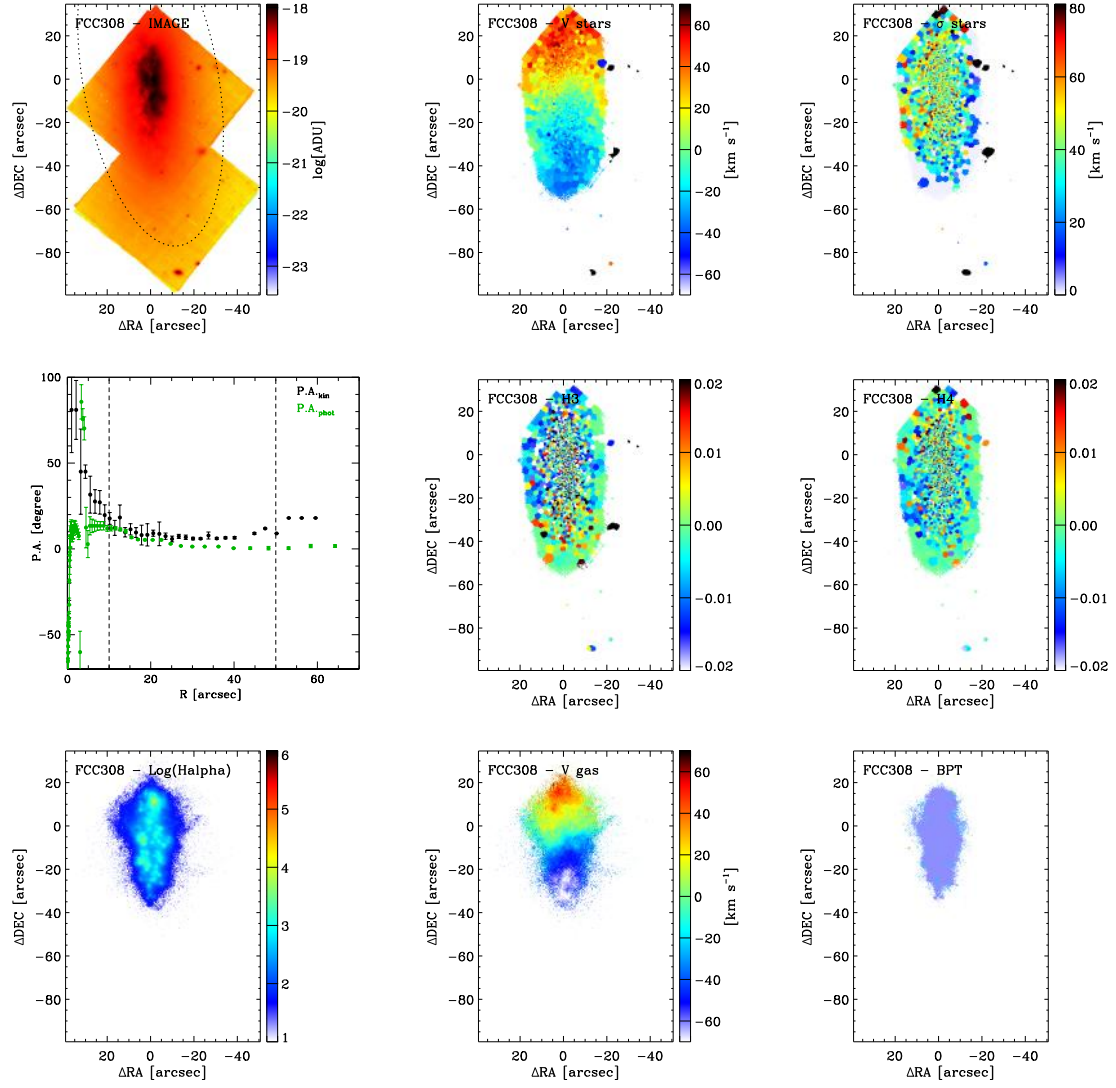
Fig. A.29. Same as in Fig. A.14, but for FCC 308.
