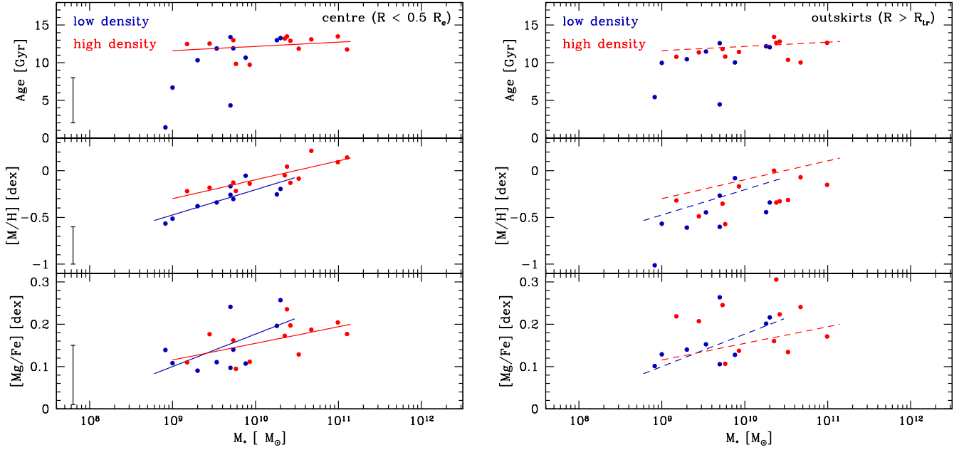
Fig. 5. Left: mean age (top), total metallicity [M/H] (middle), and [Mg/Fe] abundance ratio (bottom) in the central parts of the F3D ETGs located in the high (red circles) and low-density region (blue circles) of the cluster as a function of the total stellar mass. The red and blue lines in the middle and bottom panels are the least-square fits of the values for the central parts of the ETGs in the high and low-density regions of the cluster, respectively. The error bars in the low-left corner indicate the average uncertainty derived for each quantity. Right: same as in the left panels but for the outskirts of the F3D ETGs. The least-square fitting lines of the left panels are shown as dashed lines for comparison.
