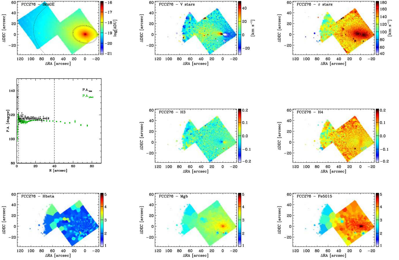
Fig. A.23. Same as in Fig. A.1, but for FCC 276.
