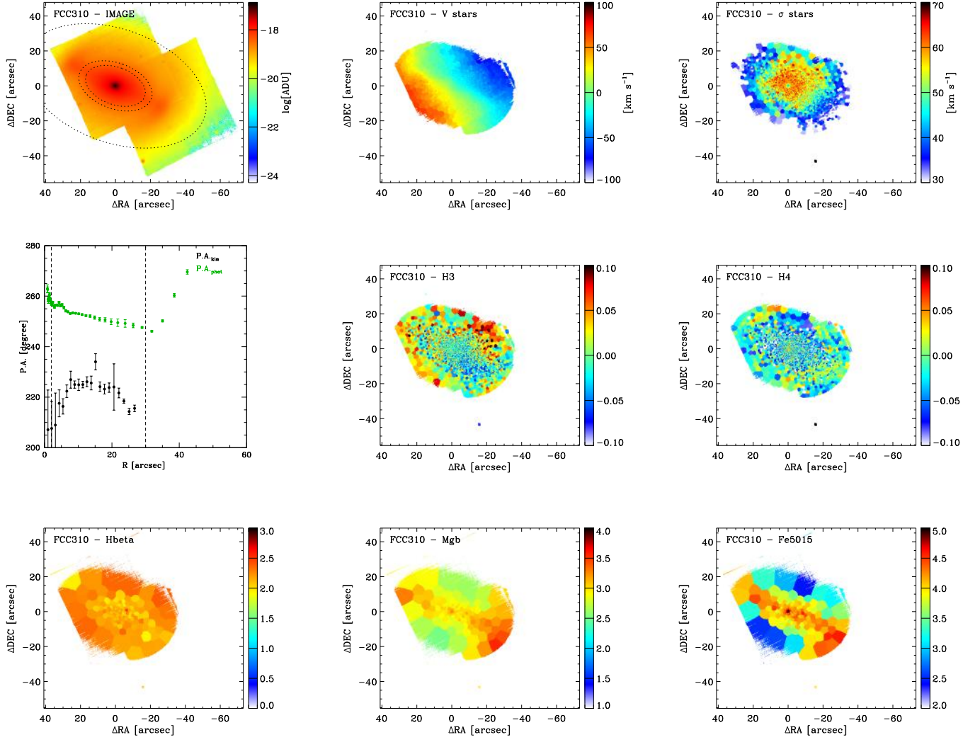
Fig. A.30. Same as in Fig. A.1, but for FCC 310.
