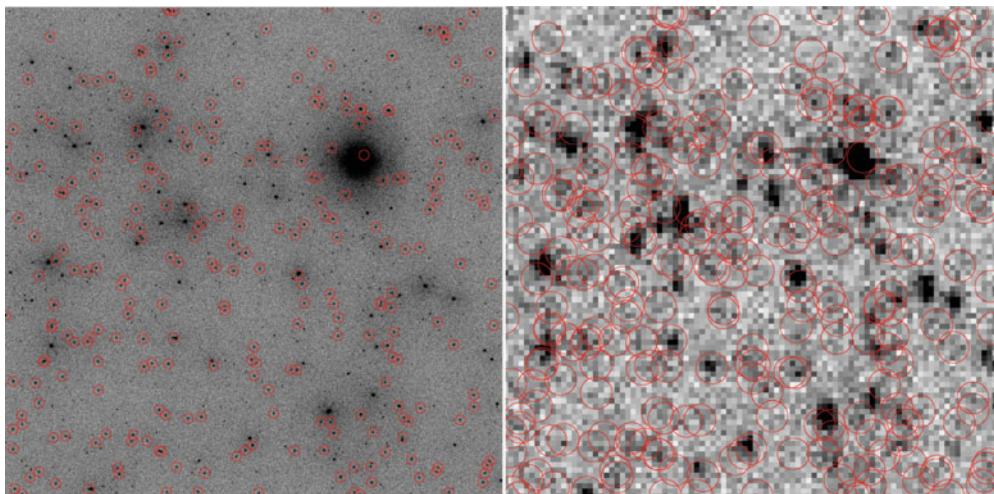
Figure 2. MICADO (left) and NIRC2 (right) 3 \times 3 arcsec 2 I -band simulated images of a stellar population typical for a stream in a galaxy halo at 8 Mpc distance (see text). A total integration time of 3 hrs has been adopted. Circles, with a diameter of 10 (left) and 6 (right) pixels, show the position of red clump stars ( 28.5 \leq I \leq 29.5 ).
