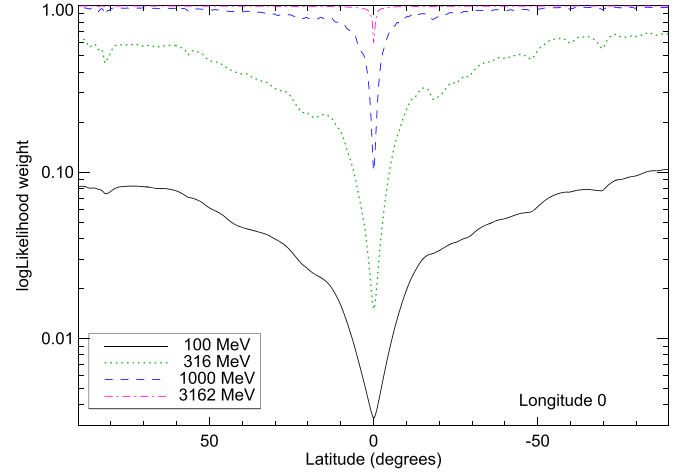
Figure 22. Data-based log-likelihood weights as a function of latitude across the Galactic Center, at 100 MeV, 300 MeV, 1 GeV, and 3 GeV, assuming all events are used throughout, and the same zenith cut at 105^\circ . The dips at some latitudes are point sources, which are included in the data-based weights. Those weights were not used in 4FGL (which uses separate event types), they are shown here only for illustration.
