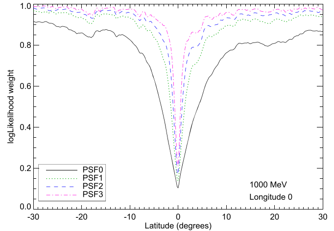
Figure 24. Data-based weights at 1 GeV for ZMax = 105^\circ as a function of latitude (for the interesting [-30^\circ, 30^\circ] region) across the Galactic Center, for different PSF event types, computed according to Equation (20). These weights were actually used in 4FGL. The average (over event types) weight is larger than the weight using all events together at the same 1 GeV energy (blue dashed line in Figure 22). This is because keeping event types separate is more favorable than merging them and losing the event type information.
