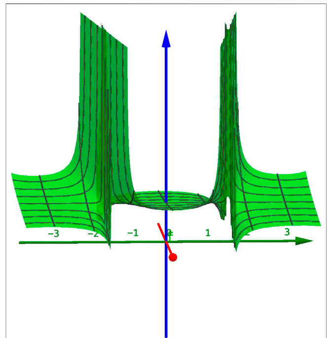
FIGURE 9 | The tomogram of a classical de Sitter universe.
