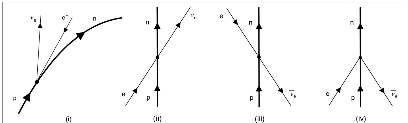
FIGURE 6 | Proton decay in the laboratory (i) and comoving (ii, iii, iv) frames (time is on the vertical axis).
