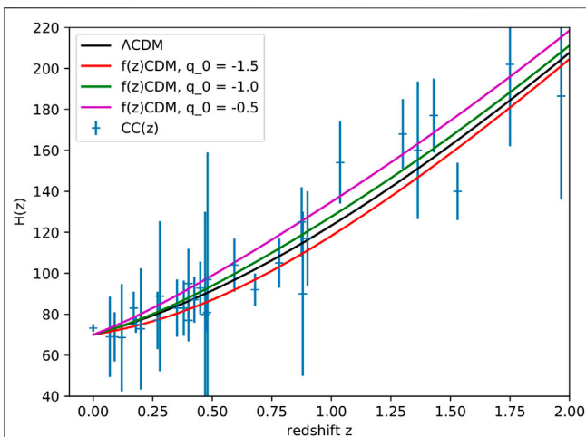
FIGURE 2 | H(z) evolution expansion of f(z) CDM model, where j_0 = 1.97 and s_0 = l_0 = 0 with different values of deceleration parameter: q_0 = -0.5 (magenta curve), q_0 = -1 (green curve), q_0 = -1.5 (red curve). For comparison, the minimal \Lambda CDM model is also drawn (black solid line) and the Cosmic Clock data are reported (see ref. 41). Moreover, \Omega_m = 0.3 , \Omega_\Lambda = 1 - \Omega_m , and H_0 = 70 Km/s/Mpc.
