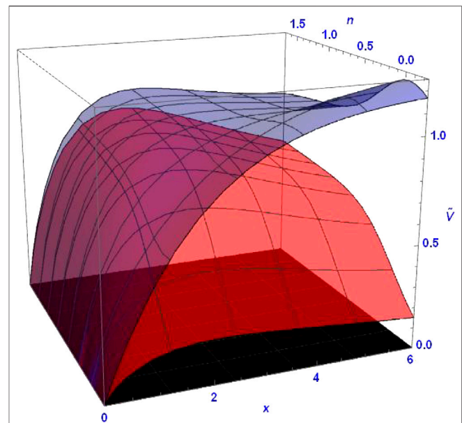
FIGURE 14 | The observed Universal Rotation Curve (blue surface) of Spirals and its Luminous Matter component (red surface). x \equiv R/R_D , with R_D the disk length-scale, \tilde{V} is the double normalized URC: \tilde{V} \equiv V(x, M_h)/V(3, M_h) with M_h the galaxy halo virial mass and: M_h = 10^{11+n} M_\odot . The discrepancy implies the presence of a dark massive component (see ref. 332).
