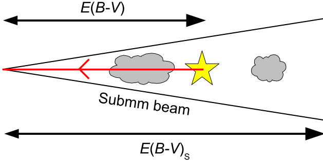
Fig. 1. Instrumental-beam and line-of-sight components affecting the comparison of polarized emission with interstellar polarization from differential extinction of a star. E(B-V) is the colour excess to the star, while E(B-V)_s is the submillimetre optical depth converted to a colour excess (Sect. 3.3).
