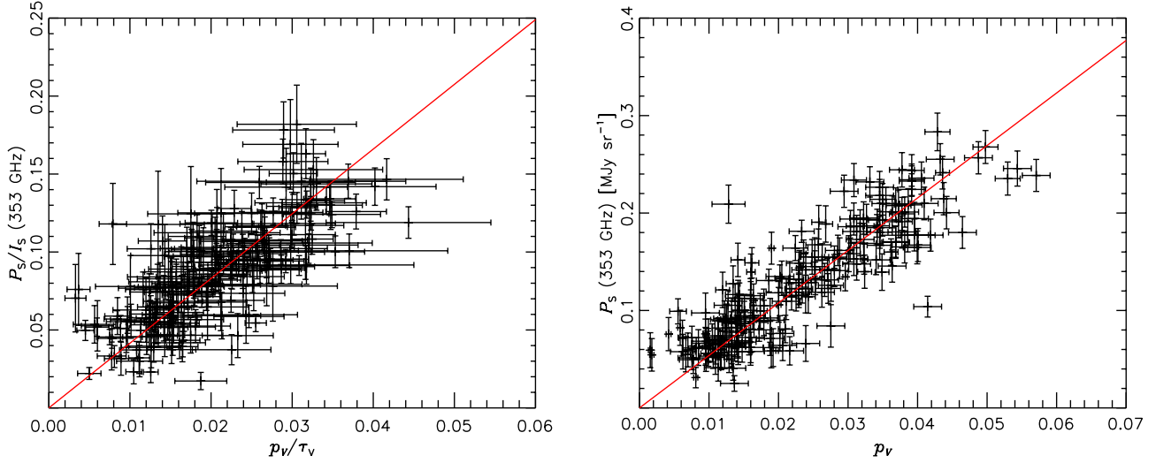
Fig. C.3. Left: correlation of debiased polarization fraction in emission with that in extinction (Pearson coefficient 0.74). Right: correlation of the debiased polarized emission (in MJy sr -1 ) with starlight polarization degree (Pearson coefficient 0.87). The range corresponds to one quadrant in Fig. 7. The fits are forced to go through the origin and have slopes R_{S/V} = 4.18 \pm 0.04 ( \chi^2_r = 1.77 ) and R_{P/p} = (5.41 \pm 0.04) MJy sr -1 ( \chi^2_r = 2.98 ), respectively.
