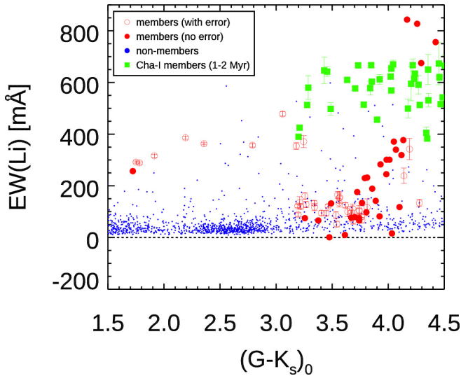
Figure 1. \text{EW}(\text{Li}) versus (G - K_s)_0 in NGC 2232, using \text{EW}(\text{Li}) measurements from GESiDR5. Red symbols represent the 80 high probability members ( P_{3D} > 0.95 ). Open and filled symbols denote \text{EW}(\text{Li}) values with and without reported uncertainties in GESiDR5, respectively. Blue points are likely non-members of NGC 2232 ( P_{3D} < 0.1 ) observed in the same instrument configurations as the members. The green squares are members of the \sim 2 Myr Cha I association also observed as part of GES.
