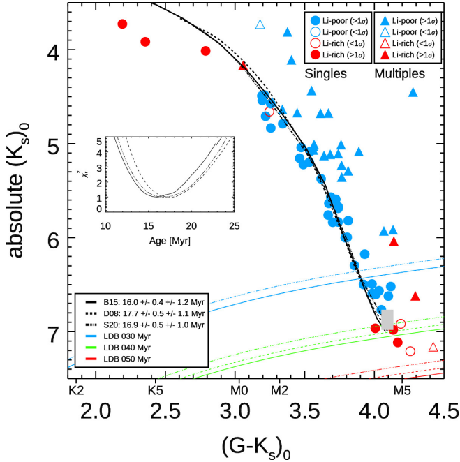
Figure 4. M_{K_s} vs (G - K_s)_0 for high probability cluster members. Red and blue symbols denote targets classed as Li-rich and Li-poor (in §4.1), where open and closed symbols denote whether the \text{EW}(\text{Li}) is within, or not within, one error bar of 300 \text{ mÅ} . Circles and triangles represent the likely-single and likely-multiple stars (in §5), respectively. The grey box denotes the estimated position of the lithium depletion boundary (LDB). The blue, green and red lines represent curves of constant luminosity at 99 per cent Li depletion from three standard models (see §4.2 for details) at 30, 40 and 50 Myr, respectively. The black curves are the best-fitting M_{K_s} vs (G - K_s)_0 isochrones to the likely single stars for the same models. The inset plot shows the reduced \chi_r^2 as a function of isochrone age.
