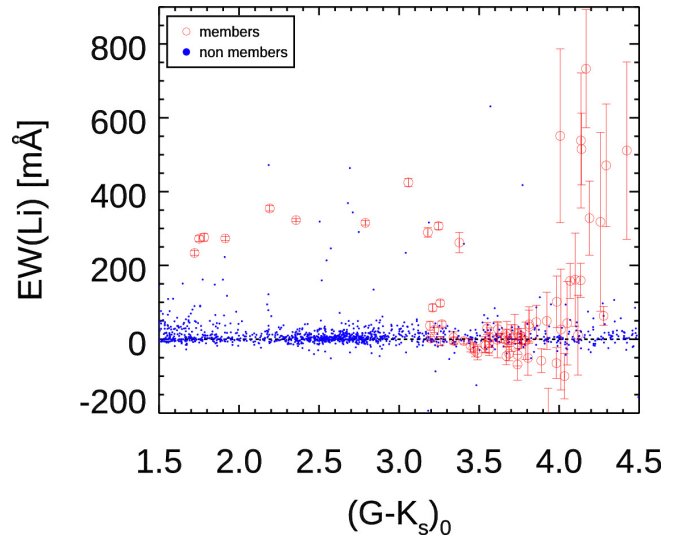
Figure 2. \text{EW}(\text{Li}) versus (G - K_s)_0 , using the revised \text{EW}(\text{Li}) values (and errors) calculated from our analysis in §3.2. The symbols and notation are the same as those described in Figure 1.
