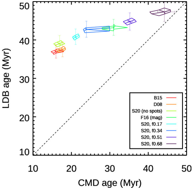
Figure 6. A comparison of the LDB- and CMD-derived ages from each model. Vertical and horizontal error bars represent the age error due to statistical uncertainty and the grids demonstrate the effect on the derived age when altering E(B-V) and d_{\text{mod}} by their error bars (representing systematic uncertainties). The dotted line denotes equivalence.
