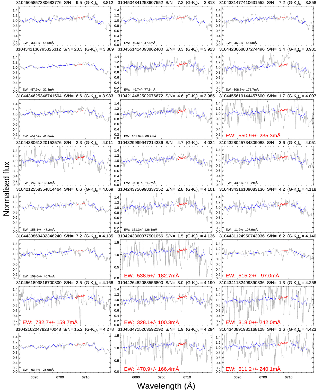
Figure 3. GES spectra for the 24 targets with (G-K_s)_0 > 3.8 . The normalised, reduced spectra from GESiDR5 are displayed in grey, where the data have been binned by 7 pixels. The best-matching spectral template (described in §3.2) is shown in the region encompassing the Li-feature at 6708 Å (in red) and in two regions either side of the feature (in blue). The title of each panel gives the Gaia DR2 source identifier, the SNR given in GESiDR5 and the (G-K_s)_0 colour. The EW(Li) values are provided in the bottom-left of each panel, where targets defined as Li-rich are highlighted in larger red text.
