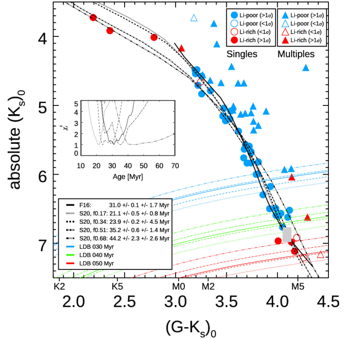
Figure 5. Similar to Fig. 4 but showing the loci of constant luminosity for 99 per cent Li depletion (coloured lines), the best fitting isochrones (black lines) and \chi_r^2 vs age for a series of magnetic models (see §4.2).
