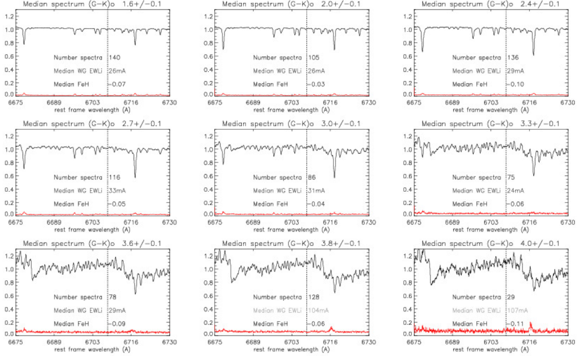
Figure B2. Examples of median continuum spectra for stars with low levels of Li as a function of (G - K_s)_0 . Text on each plot shows the number of spectra averaged in each bin and median values of EW(Li) and [Fe/H]. The lower red curve shows the uncertainty in the continuum waveform, calculated as 1.3 times the median absolute deviation of individual spectra from the median spectrum. The dotted line indicates the position of the Li I 6708 Å absorption line.
