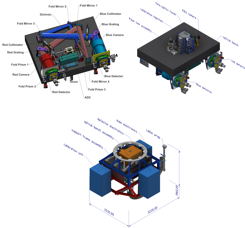
Fig. 4. Mechanical concept for CUBES: The general layout of the main mechanical components is shown. For reference, the Telescope Adapter has a diameter of about 1.5 m. The Fore-Optics Assembly is located near the center of the bench, while the spectrograph opto-mechanics are ‘hanging’ on the bottom side of the same bench.
