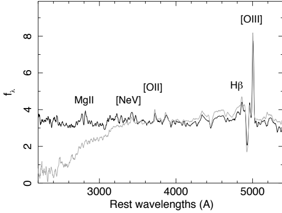
Fig. 2. UV/optical spectra of PID203, taken at the Very Large Telescope (VLT) with the FORS spectrographs (Szokoly et al. 2004). The horizontal axis is the rest-frame wavelengths in Å, assuming the galaxy redshift of z = 0.544 . The flux density f_\lambda is in units of 10^{-17} \text{ erg cm}^{-2} \text{ s}^{-1} \text{ Å}^{-1} . The data were taken on two occasions; 2000 Oct. 28 (black line) and 2000 Nov. 23 (grey line). The spectrum became redder in the second observation than in the first observation.
