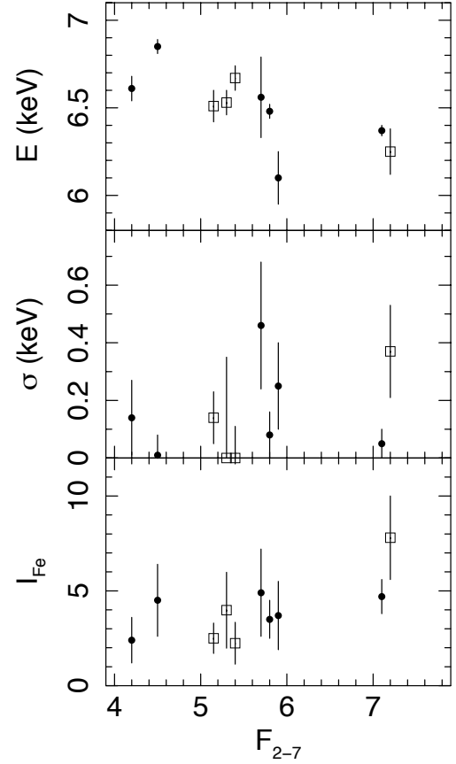
Fig. 18. Fe K line parameters of PID 319 measured in the six XMM (filled circles) and four Chandra (open squares) intervals plotted against the 2–7 keV flux in units of 10^{-14} \text{ erg s}^{-1} \text{ cm}^{-2} . The \chi^2 values against a constant hypothesis are 112.0 for the line centroid, 10.1 for the line width, and 10.0 for the line flux, respectively, for 9 degrees of freedom (the XMM-Newton and Chandra datasets combined).
