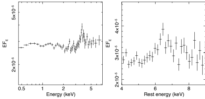
Fig. 12. Left: 0.5–7 keV spectrum of PID 319, obtained from the full exposure of three EPIC cameras. The data are plotted in flux units of EF_E as a function of energy as observed. The energy range corresponds to the rest-frame 0.87–12.2 keV. The small decline at the lowest energies is due to the Galactic absorption. The spectral flattening towards higher energies (see text) can be noticed. Right: details of the Fe K band spectrum plotted in the rest-frame 4–9 keV range. The Fe K line shows a moderately broad profile.
