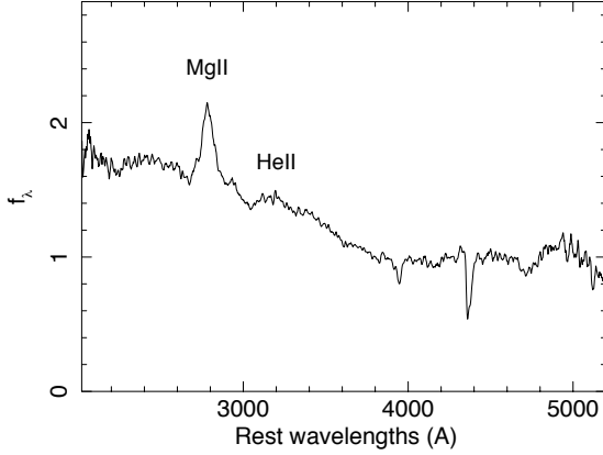
Fig. 11. UV/optical spectrum of PID319, taken at the VLT with the FORS spectrographs (Szokoly et al. 2004). The horizontal axis represents the rest-frame wavelengths in Å, assuming the galaxy redshift of z = 0.742 . The flux density f_\lambda is in units of 10^{-17} \text{ erg cm}^{-2} \text{ s}^{-1} \text{ Å}^{-1} .
