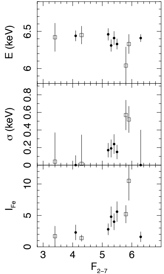
Fig. 10. Fe K line parameters of PID 203 measured in the six XMM (filled circles) and four Chandra (open squares) intervals, plotted against the 2–7 keV flux in units of 10^{-14} \text{ erg s}^{-1} \text{ cm}^{-2} . A significant (>99% confidence level) variability in line flux is observed.
