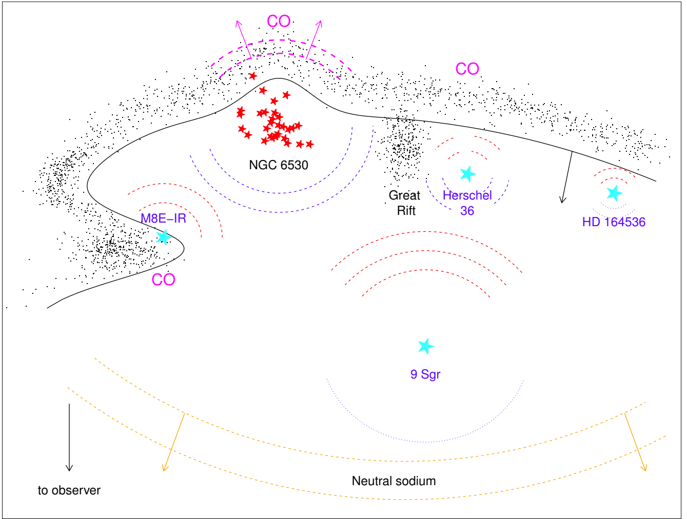
Fig. 31. Schematic representation of the Lagoon nebula geometry, along a direction passing through M 8E-IR and the Hourglass nebula. The black line indicates the molecular cloud boundary. Dusty regions are indicated with dots. Red (blue) dashed arcs indicate redshifted (blueshifted) ionized gas. Triple arcs indicate more conspicuous emission, single arcs weak emission; broken arcs indicate irregular shells. The position and motion of the known CO clouds is indicated in magenta. The most massive stars and the NGC 6530 cluster core are indicated with cyan and red stars respectively. The large-scale sodium layers are also shown (yellow dashed lines), probably not to scale.
