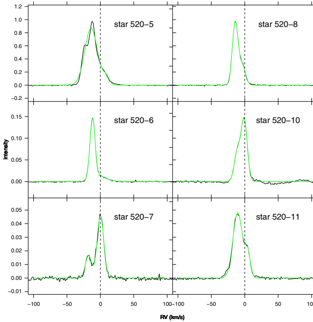
Fig. 12. Additional [O III] line examples, as in Fig. 11. Star 520-5 is the O star Her 36, the only case in which the two-Gaussian profile fails to match well the observed profile.
