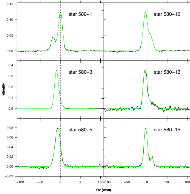
Fig. 11. Line profiles (black) and 2-g best-fit models (green) for the [O III] 5007 line, from UVES stellar spectra.
