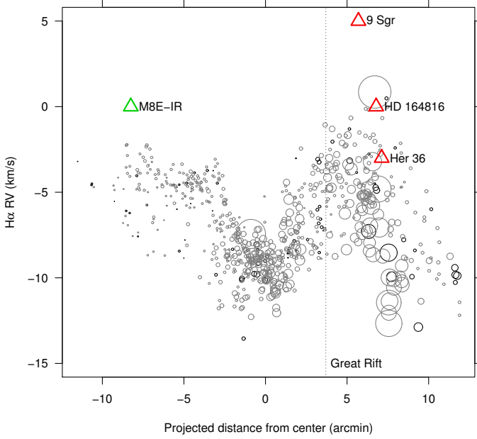
Fig. 22. Position-velocity diagram for H \alpha , inside the cluster core region (red dashed circle in Fig. 16). The projected distances in the abscissae are computed along the direction of the arrow also shown in Fig. 16. RVs from 1-g fits. Symbol size is proportional to line intensity from 1-g fits. Black (gray) circles refer to pure-sky (faint-star) fibres. The O star HD 164816 and the massive object M 8E-IR (triangles), for which no RV measurements are available, are plotted at RV = 0 , that is the NGC 6530 cluster velocity, while the other triangles indicate massive-star RVs as reported in Table 1.
