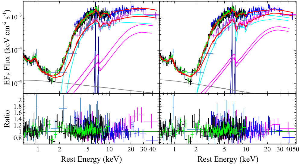
Figure 8. Best-fitting MYTorus decoupled mode (model C), applied to slice A and slice B where the left-hand panel shows a variable transmitted N_{H,Z} (and constant wind), whereas the right-hand panel shows a constant transmitted N_{H,Z} (and variable wind). Only the latter is able to fully account for the pronounced spectral curvature seen up to 40 keV in slice B. Note that for plotting purposes we adopted the combined NuSTAR FPMA+FPMB spectra. As the soft X-ray model components such as MEKAL and XSTAR emissions are not variable and do not affect the MYTorus parameters, we omitted them here for clarity. The distant scattered component is shown in grey and the MYTorus components are defined as in Fig. 7.
