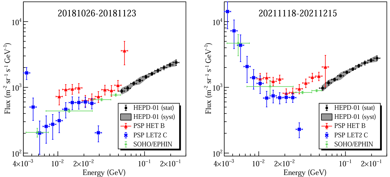
Figure 5. GCR proton spectra by HEPD-01 between 2018 October 26 and 2018 November 23 (left panel) and between 2021 November 18 and 2021 December 15 (right panel), together with proton data—in the same time intervals—from the EPHIN detector on board SOHO and the IS \odot IS suite on board the Parker Solar Probe.
