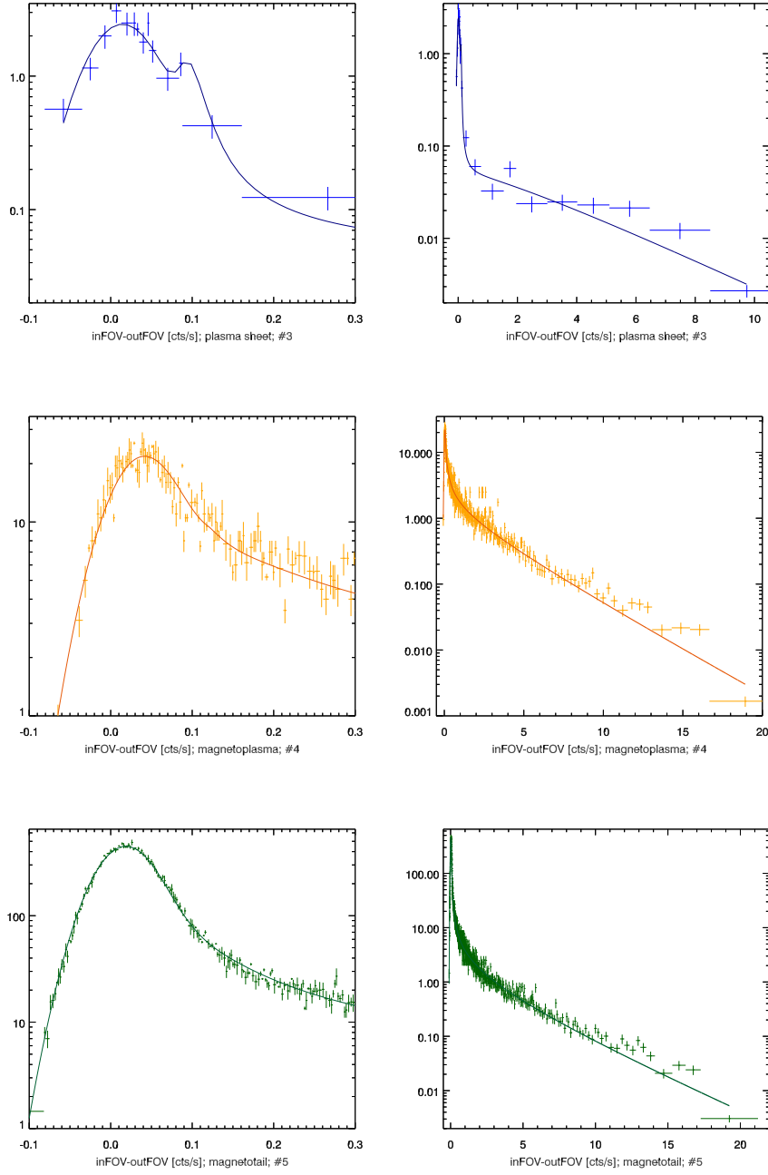
Fig. 4: inFOV-outFOV distributions of all the magnetozones. Distributions in the left column are zoomed in the range [-0.1, 0.3] for a better visualization of the low-intensity component. Best fit functions (see text) are overplotted. Different regions are color coded as in Figure 1. (Continues in next page)
