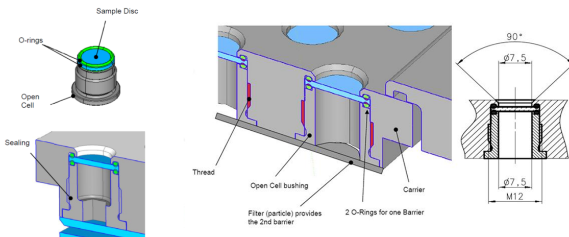
Figure 7: When open cells are used, samples are deposited on a \text{MgF}_2 disc which is accommodated in a sample carrier and held by a bushing screwed from below. The organic sample is deposited onto the inside face of the window. Picture courtesy of Kayser-Threde GmbH/RUAG.
