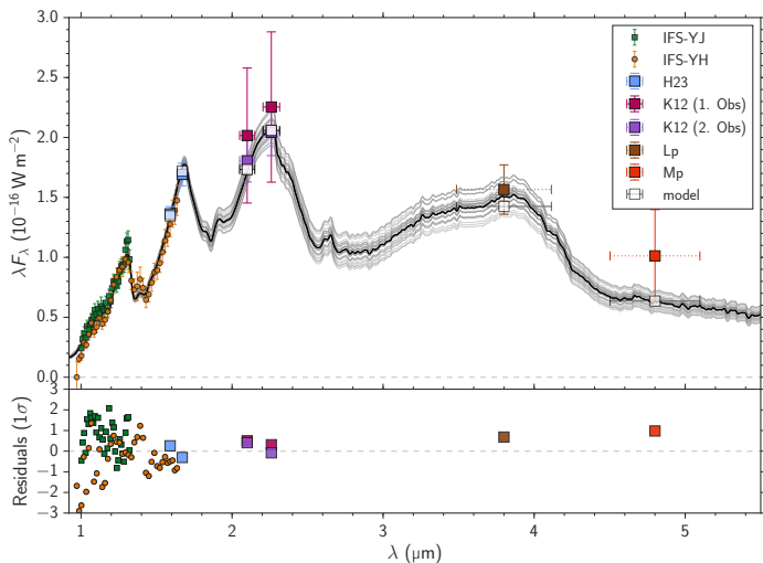
Fig. 4. The observed spectrum of HIP 65426 b (coloured squares) compared to the best-fit spectral model from the BT-Settl grid, with T_{\text{eff}}=1618\text{ K} , \log g = 3.78 and R = 1.17R_{\odot} . The horizontal error bars show the width of the SPHERE and NACO filters, and the grey squares show the predicted flux calculated using the filter transmission curves. Several models drawn from the MCMC posterior distributions are also shown in grey.
