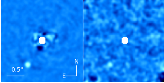
Fig. 1. Final PSF-subtracted images from the two NACO datasets in L' (left) and M' (right). The companion is detected in both datasets. While we find a lower contrast ratio in M' , the high thermal background leads to a lower overall SNR.
