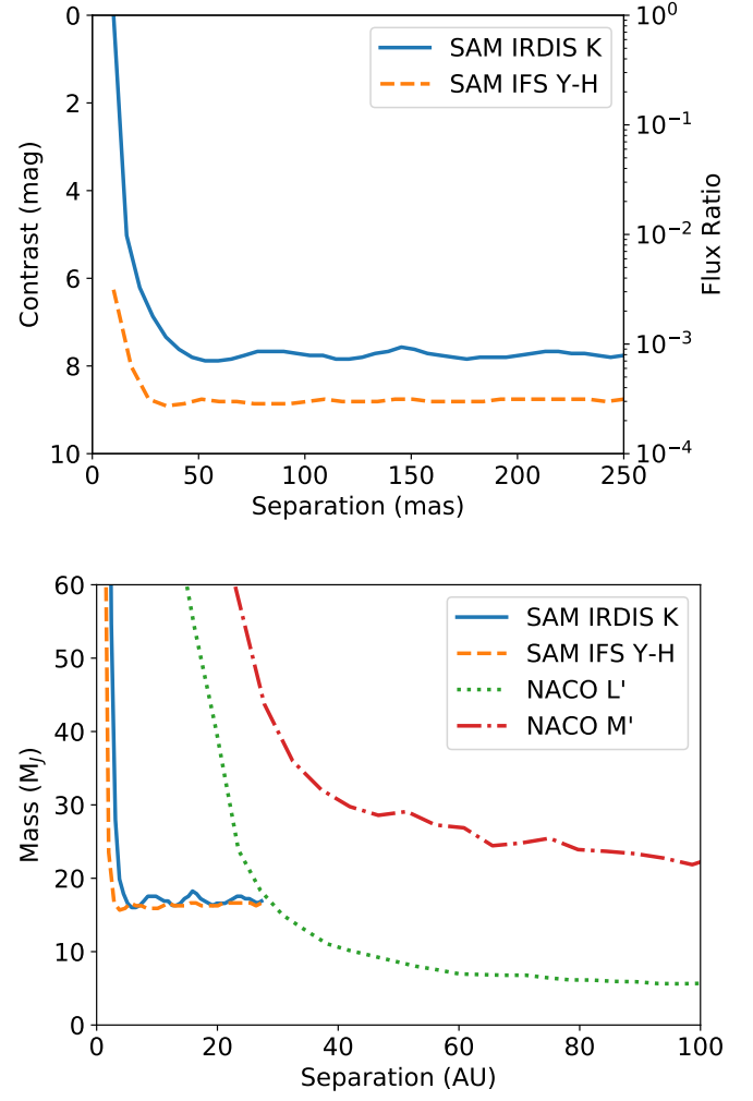
Fig. 7. Detection limits on further companions around HIP 65426. Top: Detection limits from the SPHERE-SAM data in contrast and angular separation. Bottom: Mass limits for the SPHERE-SAM and NACO data expressed as projected physical separations. The limits in contrast were converted to masses using the DUSTY isochrones.
