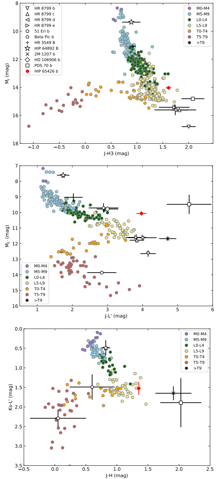
Fig. 5. Colour-magnitude and colour-colour diagrams showing the sequence of field dwarfs (coloured circles), a range of young, imaged brown dwarf and exoplanet companions (black symbols) and HIP 65426 b (red circle). HIP 65426 b falls near objects with mid-L spectral types, but is more luminous and with redder colours than the field sequence. This matches the trend seen for other young objects with similar spectral type.
