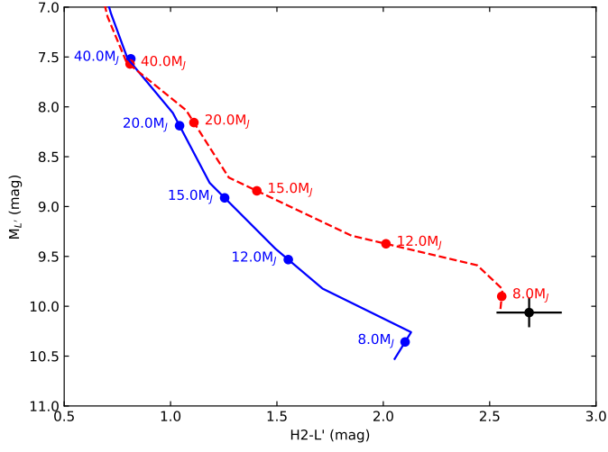
Fig. 6. Colour-magnitude diagram showing the COND (blue) and DUSTY (red) evolutionary models compared to HIP 65426 b. We find that the colours of HIP 65426 b match the DUSTY models more closely than the COND predictions.
