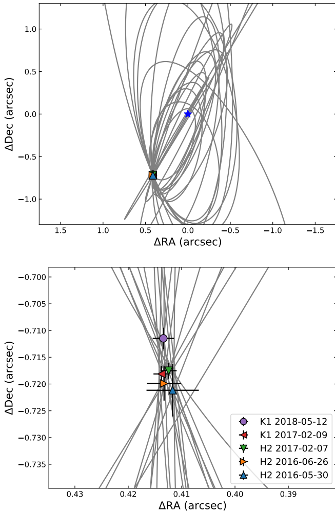
Fig. 2. The observed SPHERE-IRDIS astrometry of HIP 65426 b compared to 20 orbits drawn randomly from the 250 best-fitting orbits in the OFTI output sample. The position of the primary star is shown with a blue star. A close up of the region around the present position of HIP 65426 b is shown separately in the bottom plot.
