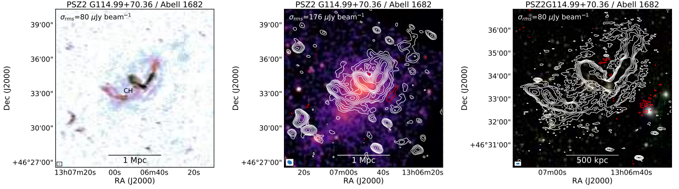
Fig. A.9. PSZ2 G114.99+70.36, Abell 1682. Left: robust -0.5 radio image. Middle: Chandra X-ray image with 10'' tapered radio contours. Right: optical image with robust -0.5 image radio contours. For more details, see the caption of Fig. 5.
