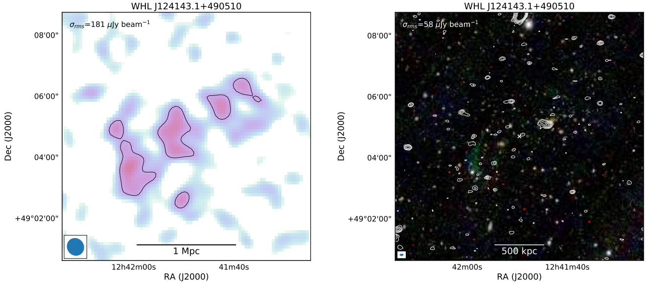
Fig. 21. WHL J124143.1+490510. Left: 30'' tapered radio image with compact sources subtracted. Right: optical image with robust -0.5 image radio contours. For more details, see the caption of Fig. 5.
