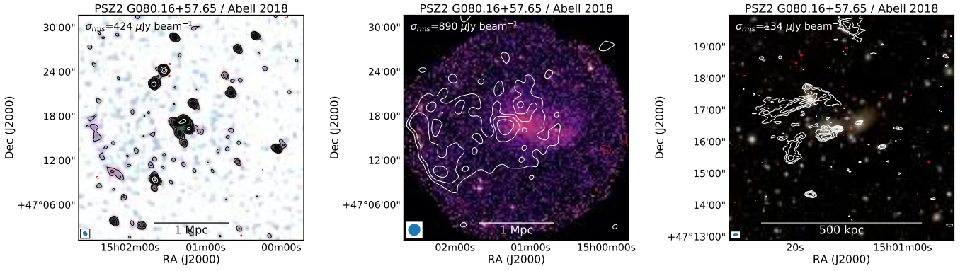
Fig. 5. PSZ2 G080.16+57.65, Abell 2018. Left: low-resolution 144 MHz radio image made with a 30'' taper. Middle: XMM-Newton image with radio contours from a 90'' tapered image overlaid. Compact sources were subtracted in this image. Right: Pan-STARRS gri color image overlaid with radio contours from the robust -0.5 weighted image. The cluster center position is marked with a white "X". Radio contours are drawn at 3\sigma_{\text{rms}} \times [1, 2, 4, \dots] , where \sigma_{\text{rms}} is the rms map noise. Negative -3\sigma_{\text{rms}} contours are drawn in red. The rms noise levels of the radio images used are provided in the top right corner of each panel.
