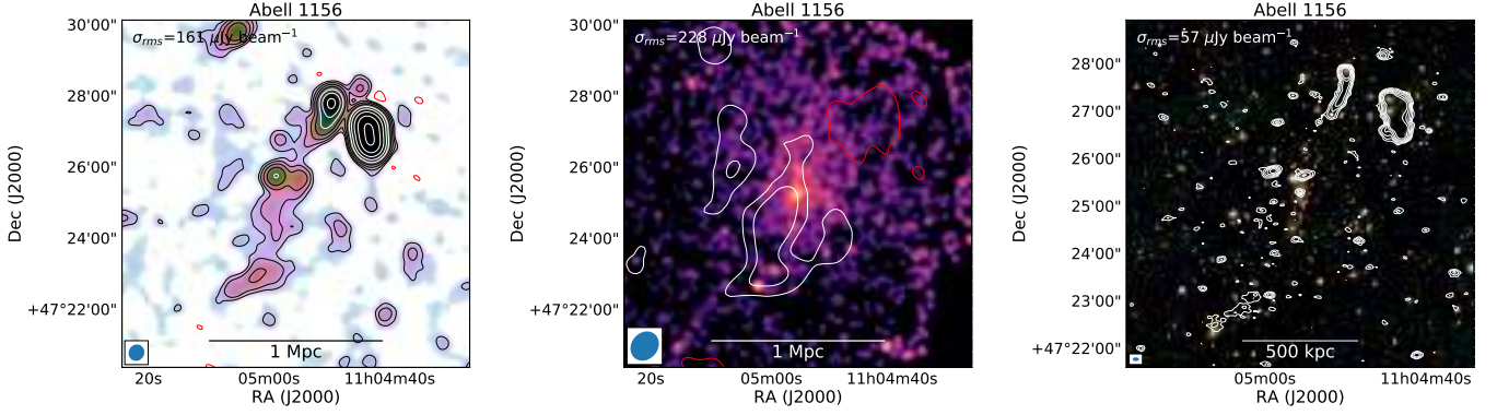
Fig. 17. Abell 1156. Left: 15'' tapered radio image. Middle: Chandra X-ray image with 30'' tapered radio contours (compact sources were subtracted). Right: optical image with robust -0.5 image radio contours. For more details, see the caption of Fig. 5.
