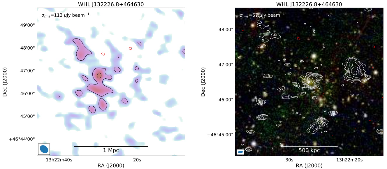
Fig. 22. WHL J132226.8+464630. Left: 15'' tapered radio image with compact sources subtracted. Right: optical image with robust -0.5 image radio contours. For more details, see the caption of Fig. 5.
