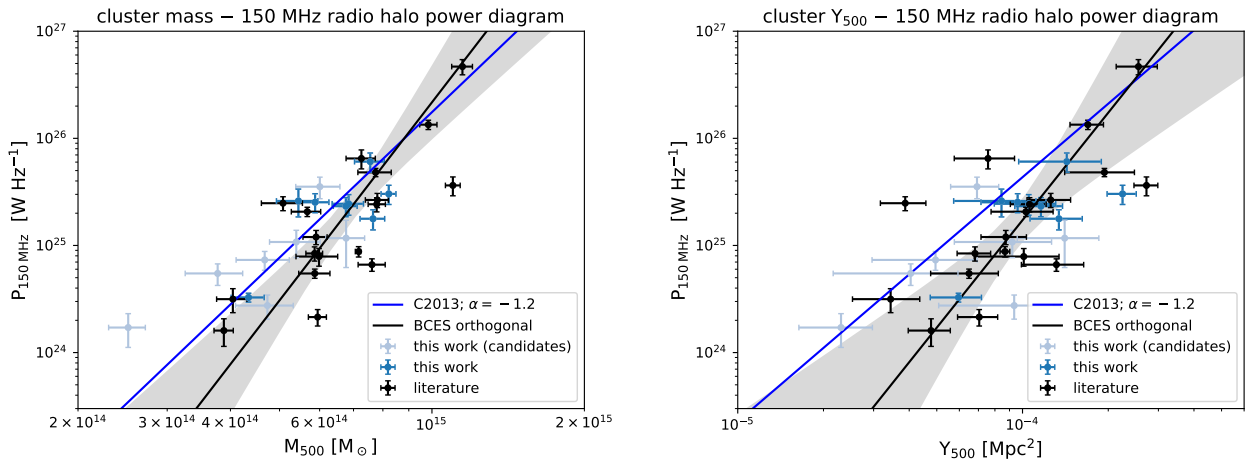
Fig. 25. Radio halo powers plotted against cluster mass proxies. Left: distribution of clusters in the mass ( M_{500} ) 150 MHz radio power ( P_{150\text{ MHz}} ) plane. The solid black line displays the BCES orthogonal fit (candidate halos were excluded). The shaded region shows the 3\sigma (99.7% confidence) region of the fit. The blue line is the BCES orthogonal fit from Cassano et al. (2013) scaled with a spectral index of -1.2 . Right: distribution of clusters in the Y_{500} 150 MHz radio power plane. The plotted symbols and lines represent the same data sets as in the left panel.
