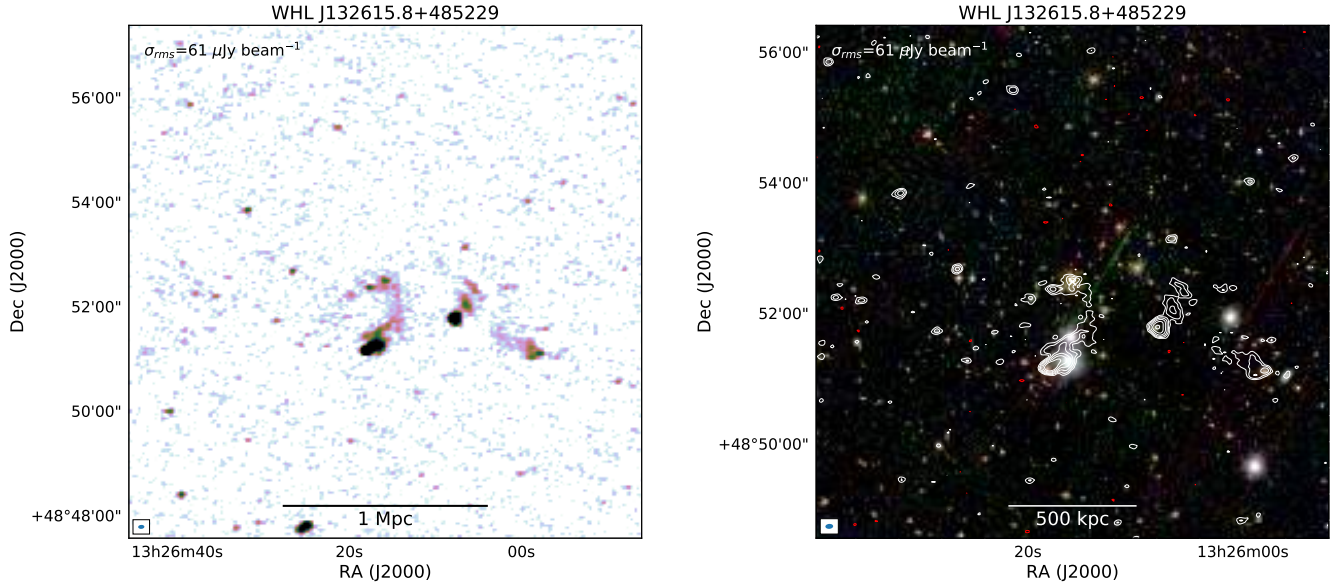
Fig. A.19. WHL J132615.8+485229. Left: robust -0.5 image radio image. Right: optical image with robust -0.5 image radio contours. For more details, see the caption of Fig. 5.
