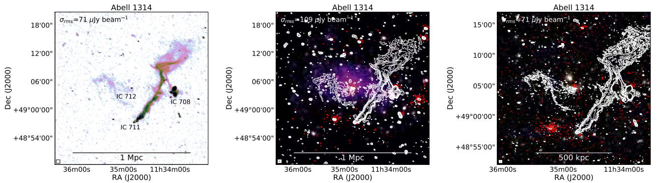
Fig. 18. Abell 1314. Left: robust -0.5 radio image. Middle: XMM-Newton X-ray image with 10'' tapered radio contours. Right: optical image with robust -0.5 image radio contours. For more details, see the caption of Fig. 5.
