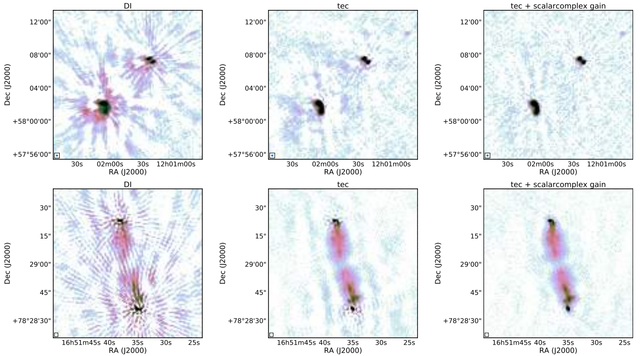
Fig. 3. Improvement during self-calibration on extracted data. Left column : starting point of this process: a DI calibrated image. Middle column : results after DPPP TEC calibration, with all LOFAR core stations forced (“antenna constraint” solve) to have the same solution. Right column : final image after DPPP scalarcomplex gain calibration. Top row : 43–67 MHz LBA data. Bottom row : LOFAR international-baseline 120–168 MHz HBA data.
