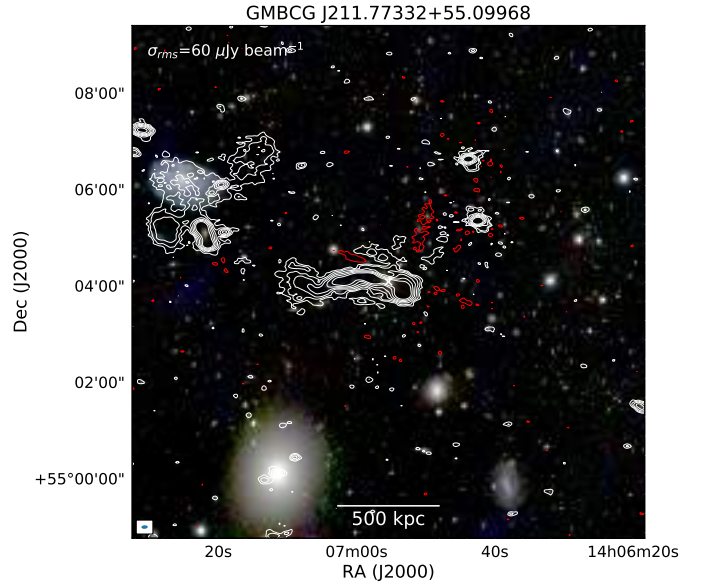
Fig. A.17. GMBCG J211.77332+55.09968. Optical image with robust -0.5 image radio contours. For more details, see the caption of Fig. 5.
