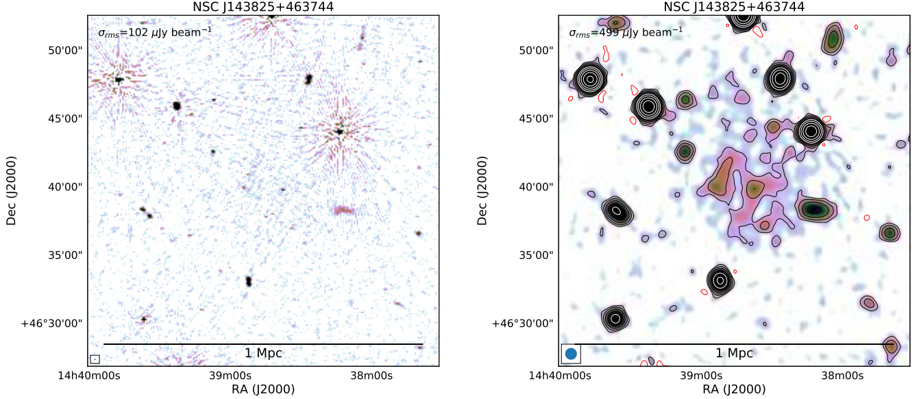
Fig. 19. NSC J143825+463744. Left: robust -0.5 radio image. Right: 30'' tapered radio image. For more details, see the caption of Fig. 5.
