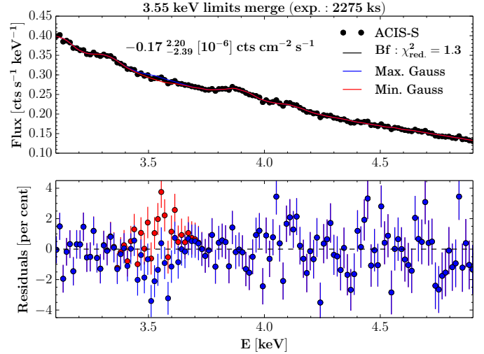
Fig. C.1. Merged X-ray spectrum (ACIS-S) of the cluster sample with residuals of different fitted models. Fitted XSPEC models: apec+apec+zgauss (3.55 keV) +zgauss (3.85 keV) +zgauss (4.7 keV) with best-fit (Bf), upper and lower confidence values (99.7 per cent) of the Gaussian flux at 3.55 keV in counts \text{cm}^{-2} \text{s}^{-1} . The annotations show the best-fit value and the confidence interval obtained using MCMC. Residuals are shown for the fit with upper (blue) and lower (red) confidence limit of the 3.55 keV Gaussian flux. For the effective area curve, see Fig. B.1.
