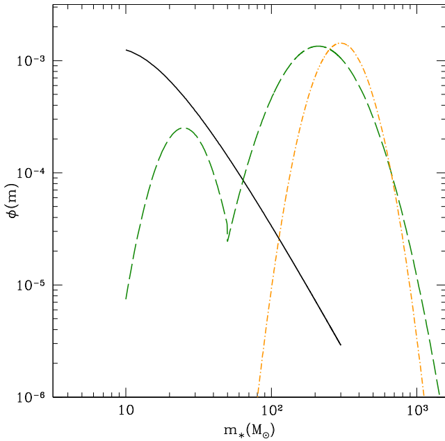
Figure 10. IMF of Pop III stars. The black solid line shows the Larson IMF adopted in the reference model, normalized to 1 in the mass range [10\text{--}300]\text{ M}_\odot . Green dashed and orange dot-dashed lines show the analytic functions used to approximate the results of Hirano et al. (2015) for J_{\text{LW}} < 0.1 and > 0.1 , respectively. In both cases, the mass distribution is normalized to 1 in the mass range [10\text{--}2000]\text{ M}_\odot .
