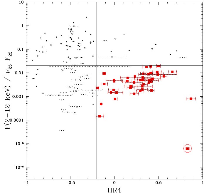
Fig. 2. F(2\text{--}12\text{ keV})/(\nu_{25}F_{25}) vs. HR4 diagnostic plot for the 145 sources found by cross-correlating the PSC IRAS catalogue at 25 \mu\text{m} and the 2XMM catalogue. Filled squares (red symbols in the electronic version only) are the 44 sources that have flux ratios and X-ray colors typical of Compton-thick AGN. The isolated object in the bottom-right part of the diagram marked with an empty circle is the only Galactic source (V*RAqr) present in the Compton-thick candidate region.
