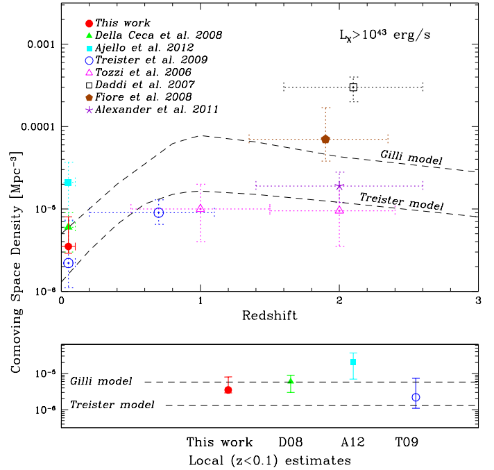
Fig. 5. Co-moving space density of Compton-thick AGN. All the data and the model plotted in the figure refer to L_X > 10^{43}\text{ erg s}^{-1} . Filled circle (red symbol in the electronic version only) is the estimate obtained in this work, while the other local values are taken from Della Ceca et al. (2008b, solid triangle, green symbol in the electronic version), from Ajello et al. (2012, solid square, cyan symbol in the electronic version) and from Treister et al. (2009a, open circle at the local redshift, blue symbol in the electronic version only). As for higher redshift estimates: open circle (blue symbol in the electronic version only), filled pentagon (brown symbol in the electronic version only) and open square are the results obtained from the X-ray stacking analysis of undetected candidate Compton-thick AGN from Treister et al. (2009b), Fiore et al. (2008) and Daddi et al. (2007), respectively. The results obtained from the X-ray spectral analysis from Tozzi et al. (2006) and Alexander et al. (2011) are marked with open triangles (magenta symbols in the electronic version only) and star (purple symbol in the electronic version only), respectively. The results are compared to the predictions of the models proposed by Gilli et al. (2007) and Treister et al. (2009a), dashed curves. The local co-moving space density estimates are reported also in the lower panel as a function of the different authors.
