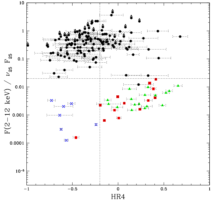
Fig. 1. F(2-12 \text{ keV})/(\nu_{25} F_{25}) vs. \text{HR}4 diagnostic plot. Filled circles (black symbol in the electronic version only) are unabsorbed and absorbed Compton-thin AGN ( N_{\text{H}} < 10^{24} \text{ cm}^{-2} ) taken from two different X-ray samples in the literature (XMM-HBS sample – Della Ceca et al. 2008b; XMDS survey – Tajer et al. 2007; Polletta et al. 2007). Stars (blue objects in the electronic version only) are a sample of local starburst galaxies (Ranalli et al. 2003) and squares (red objects in the electronic version only) and triangles (green objects in the electronic version only) are local “confirmed” and “candidate” Compton-thick AGN, respectively, taken by the compilation of Della Ceca et al. (2008a).
