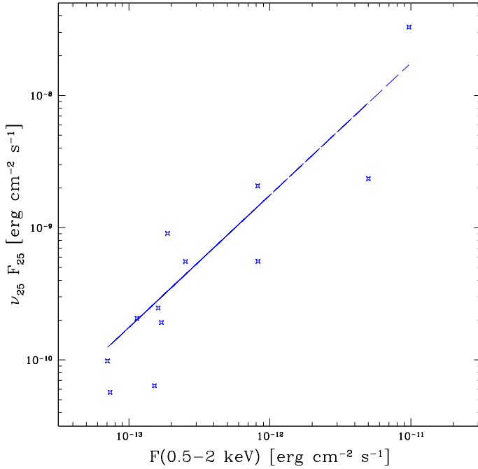
Fig. 4. Mid-IR ( \nu_{25} F_{25} ) vs. X-ray ( F(0.5\text{--}2\text{ keV}) ) fluxes of the sources populating the lower-left region in Fig. 2 after excluding the sources classified as “Seyfert”, “LINERs” or “Star” by NED. The straight line (blue line in the electronic version only) indicates the mean value of the \nu_{25} F_{25}/F(0.5\text{--}2\text{ keV}) of these sources.
