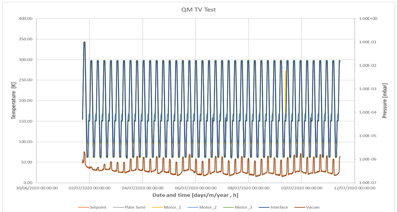
Figure 8: Temperature and vacuum plots for the QM test
