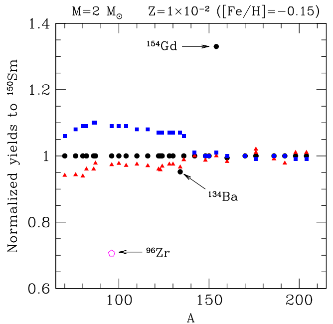
Figure 15. Differences in the yields of a 2 M_{\odot} model with Z = 10^{-2} ( [\text{Fe}/\text{H}] = -0.15 ) obtained by varying strong and weak reaction rates (dots: variations of nuclear process efficiencies in correspondence to ^{134}\text{Cs} and ^{154}\text{Eu} branching; triangles: variations of neutron source cross sections; squares: variations of neutron poison cross sections). Differences are normalized to variations in ^{150}\text{Sm} yields. See text for details.
