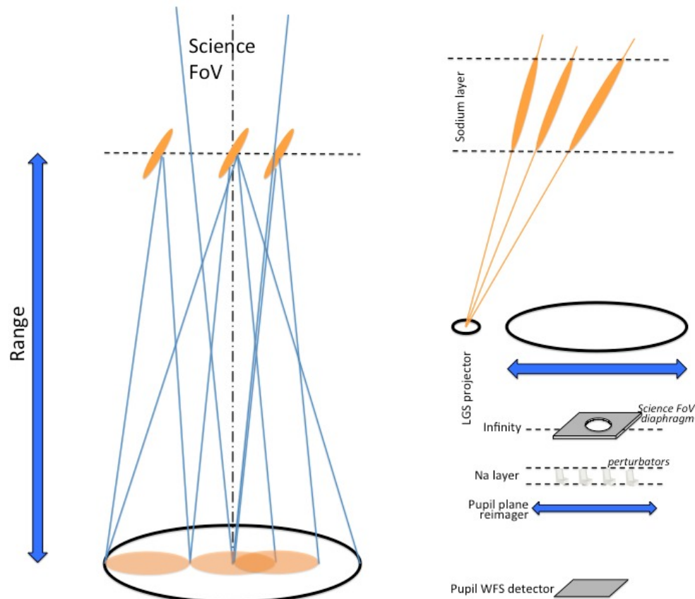
Figure 3 On the right side an illustrative way on how rays are selected in order to match the required scientific FoV. Pupil coverage depends upon the size of such diaphragms in a way that a smaller FoV would requires a larger density of beacons. Proper choice should be given to the number and density of these as depicted in the illustrative example on the left side where two pupil patches just smack each other or exhibits a significant overlap for a proper stitching.
