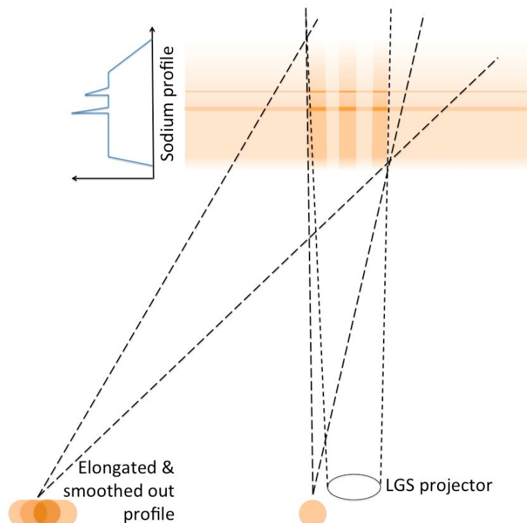
Figure 1 - In this simplified scheme it is shown that the structure of an LGS, both because of the upward turbulence and because of the Sodium density profile, will appear as elongated and smoothed out.
