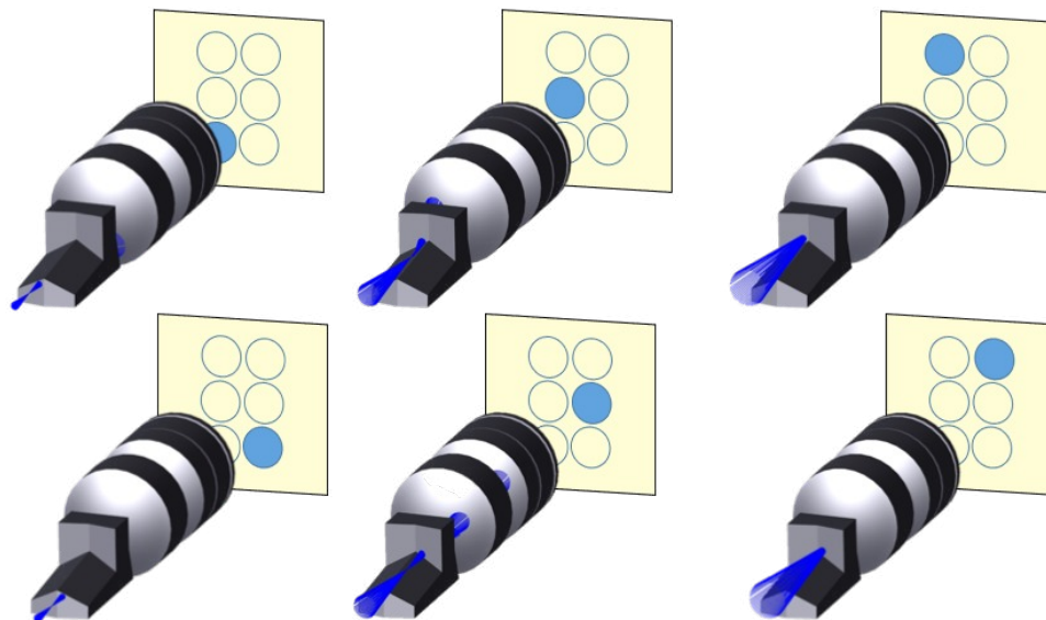
Figure 2 In this figure an ingot WFS is shown with the LGS light coming from the lower left side, away from the focal plane where NGS are focused. Depending upon the relative position along the prism all the six faces are illuminated. In contrast with the pyramid WFS, and also because of the extended nature of the reference, the illumination of the six pupils under no turbulence is not uniform and reflects the different elongation as seen from different points on the pupil. For instance, in the points closer to where the LGS is propagated most of the light is split into four pupils as in the conventional pyramid, allowing for a uniform sensing on both axes.
