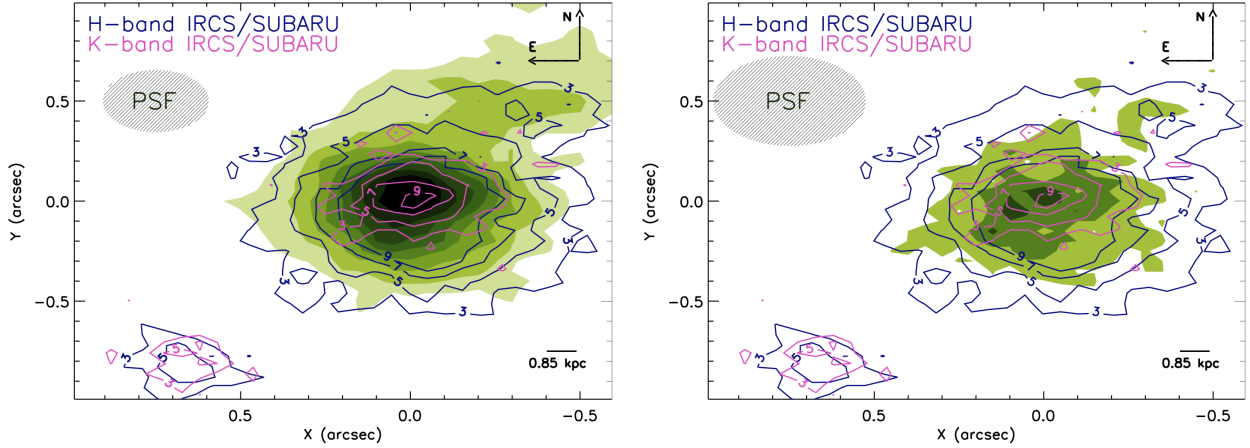
Fig. 7. Left: Contours of the Subaru/IRCS H -band (blue) and K -band (magenta) emission taken from Fig. 5 overlaid on the [O III]5007 channel map obtained integrating the SINFONI datacube on the line core ( \lambda = 1236.1\text{--}1238.9 nm; corresponding to the rest-frame range 5001–5012 Å). All contours and colour level starts from 3\sigma with steps of +2, as labelled. Spatial scale is given in arcsec. The [O III] systemic emission is overall symmetric, except for a plume extending beyond 0.5'' ( \sim 4.5 kpc) in the north-west direction. Right: same, but for the H\alpha line, collapsing the channels in the wavelength range \lambda = 1620.6\text{--}1624.0 nm (corresponding to the rest-frame range 6556–6570 Å). The same plume is also seen in the IRCS H -band data (sampling the H\alpha region), but it is not seen in the IRCS K -band data.
