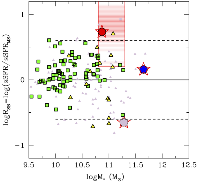
Fig. 12. Logarithm of the starburstiness, R_{SB} , defined as the ratio of the sSFR to that expected for MS galaxies as parametrised by Whitaker et al. (2012), as a function of the logarithm of the stellar mass. XID5395 is the red star. We also plot, with starred symbols, two additional sources from XMM-COSMOS for which the outflows have been revealed: XID2028 at z \sim 1.6 , from Cresci et al. 2015a, blue; and XID70135/MIRO20581 at z \sim 2.5 from Perna et al. 2015b, grey. Green squares are objects from the MASSIV survey (Contini et al. 2012) in the redshift range z = 1-2 ; yellow triangles are sources at z = 1-2 in the Genzel et al. (2014) IFU sample. We also plot, with small grey triangles, all the other sources in the Genzel et al. (2014) samples in the redshift range z = 2-3 . The shaded red region indicates the range of sSFR and stellar mass of the targets in Harrison et al. (2012).
