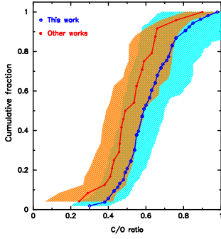
Fig. 1. Comparison between the C/Os derived in this work and those from Teske et al. (2014) and Schuler et al. (2015).
