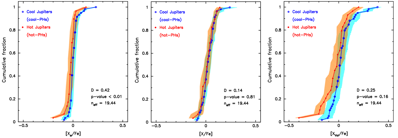
Fig. 6. Histogram of cumulative frequencies of [X_{\alpha}/Fe] (left), [X_{Fe}/Fe] (middle), and [X_{vol}/Fe] (right).
