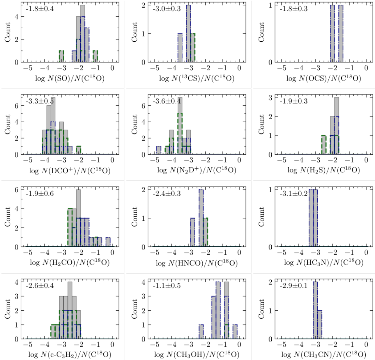
Fig. 14. Abundance histograms (relative to \text{C}^{18}\text{O} ) of all species fitted with XCLASS. The gray histogram shows the combined results of all 29 cores. The mean and standard deviation are shown in the top left corner. The green dashed and blue dash-dotted histograms show the results for the cores in ISOSS J22478+6357 and ISOSS J23053+5953, respectively.
