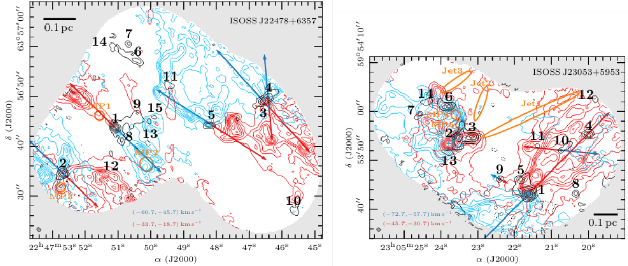
Fig. 5. CO 2–1 outflows in ISOSS J22478+6357 (left panel) and ISOSS J23053+5953 (right panel). The blue and red contours show the integrated intensity of the blue- and red-shifted line wings, respectively. The intensity is integrated over v_{\text{LSR}} - 21 to v_{\text{LSR}} - 6 and over v_{\text{LSR}} + 6 to v_{\text{LSR}} + 21 \text{km s}^{-1} for the blue- and red-shifted integrated intensity, respectively. The corresponding velocity ranges are shown in each panel. Contour levels range from 10 to 90% of the peak integrated intensity with steps of 10%. In ISOSS J22478+6357 the red- and blue-shifted peak integrated intensity is 45 and 47 \text{K km s}^{-1} and in ISOSS J23053+5953 it is 112 and 140 \text{K km s}^{-1} , respectively. Red- and blue-shifted outflow directions are indicated by red and blue arrows, respectively. The NOEMA 1.3 mm continuum data are shown in black contours. The dotted black contour marks the -5\sigma_{\text{cont}} level. Solid black contour levels are 5, 10, 20, 40, and 80\sigma_{\text{cont}} . All mm cores identified in Beuther et al. (2021) are labeled in black. Positions with a peak in molecular emission, but no associated continuum (“molecular peaks”, MP) are indicated by orange circles (Sect. 4.2.1). Jet-like structures, seen in SiO 5–4 emission, are indicated by orange ellipses (Fig. 7). The synthesized beam of the continuum data is shown in the bottom left corner. The synthesized beam of the spectral line data is similar. A linear spatial scale of 0.1 pc is indicated by a black scale bar.
