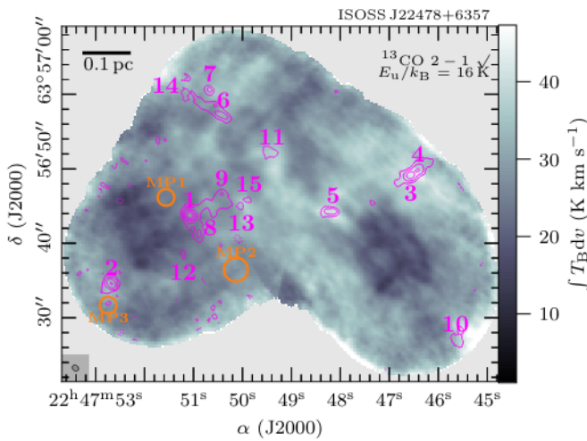
Fig. A.15. The same as Fig. 6, but for ^{13}\text{CO } 2 - 1 .
