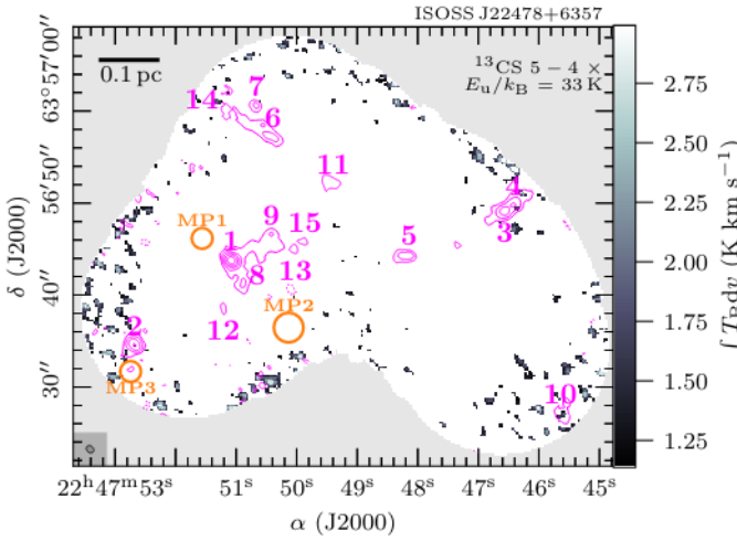
Fig. A.20. The same as Fig. 6, but for ^{13}\text{CS} 5 – 4.
