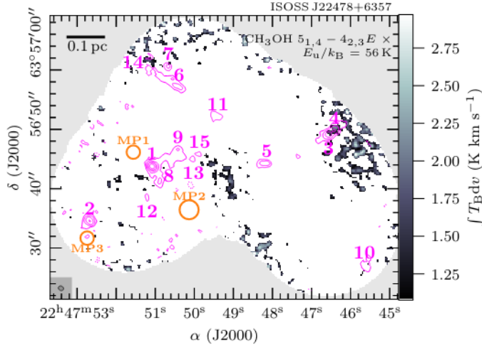
Fig. A.4. The same as Fig. 6, but for \text{CH}_3\text{OH } 5_{1,4} - 4_{2,3}E .
