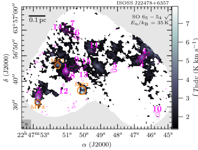
Fig. A.13. The same as Fig. 6, but for SO 6_5 - 5_4 .
