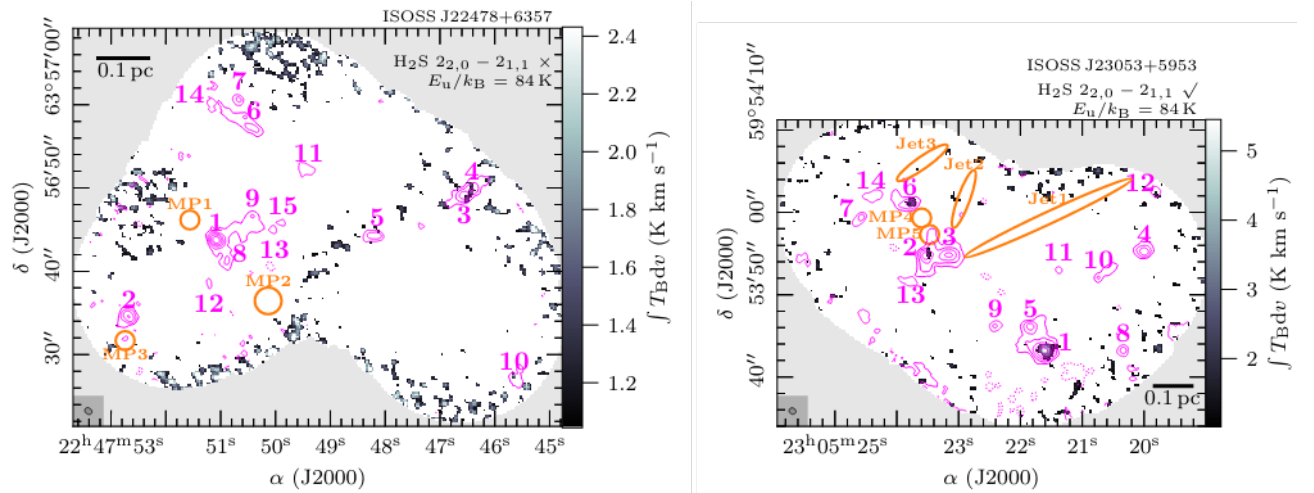
Fig. A.3. The same as Fig. 6, but for H _2 S 2_{2,0} - 2_{1,1} .
