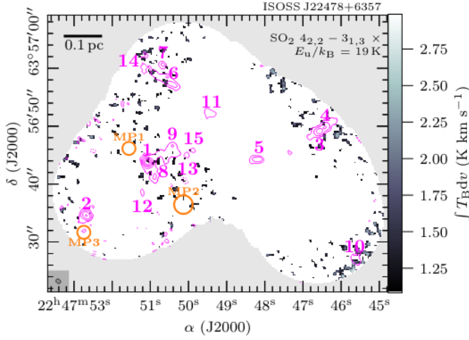
Fig. A.22. The same as Fig. 6, but for \text{SO}_2 4_{2,2} - 3_{1,3} .
