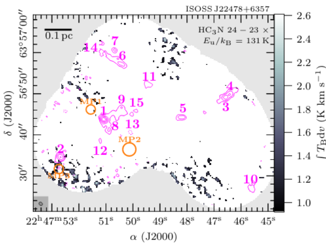
Fig. A.6. The same as Fig. 6, but for \text{HC}_3\text{N } 24 - 23 .
