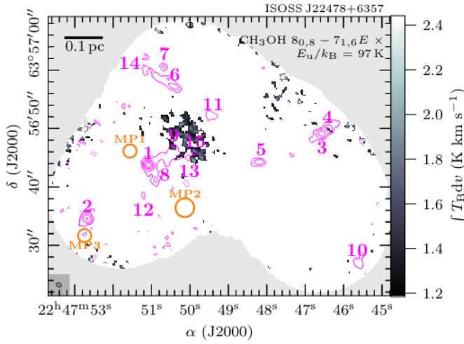
Fig. A.14. The same as Fig. 6, but for CH 3 OH 8_{0,8} - 7_{1,6} .
