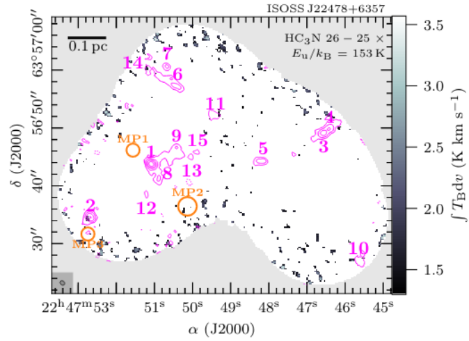
Fig. A.23. The same as Fig. 6, but for \text{HC}_3\text{N} 26 - 25 .
