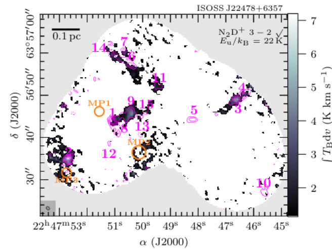
Fig. A.21. The same as Fig. 6, but for \text{N}_2\text{D}^+ 3 – 2.
