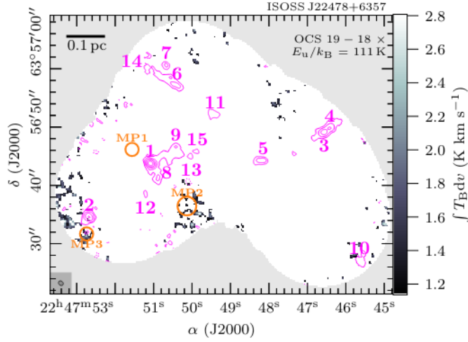
Fig. A.19. The same as Fig. 6, but for OCS 19 – 18.
