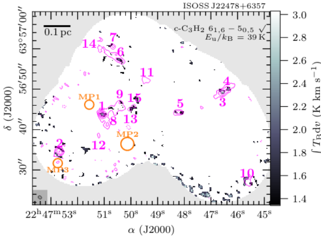
Fig. A.5. The same as Fig. 6, but for \text{c-C}_3\text{H}_2 \ 6_{1,6} - 5_{0,5} .
