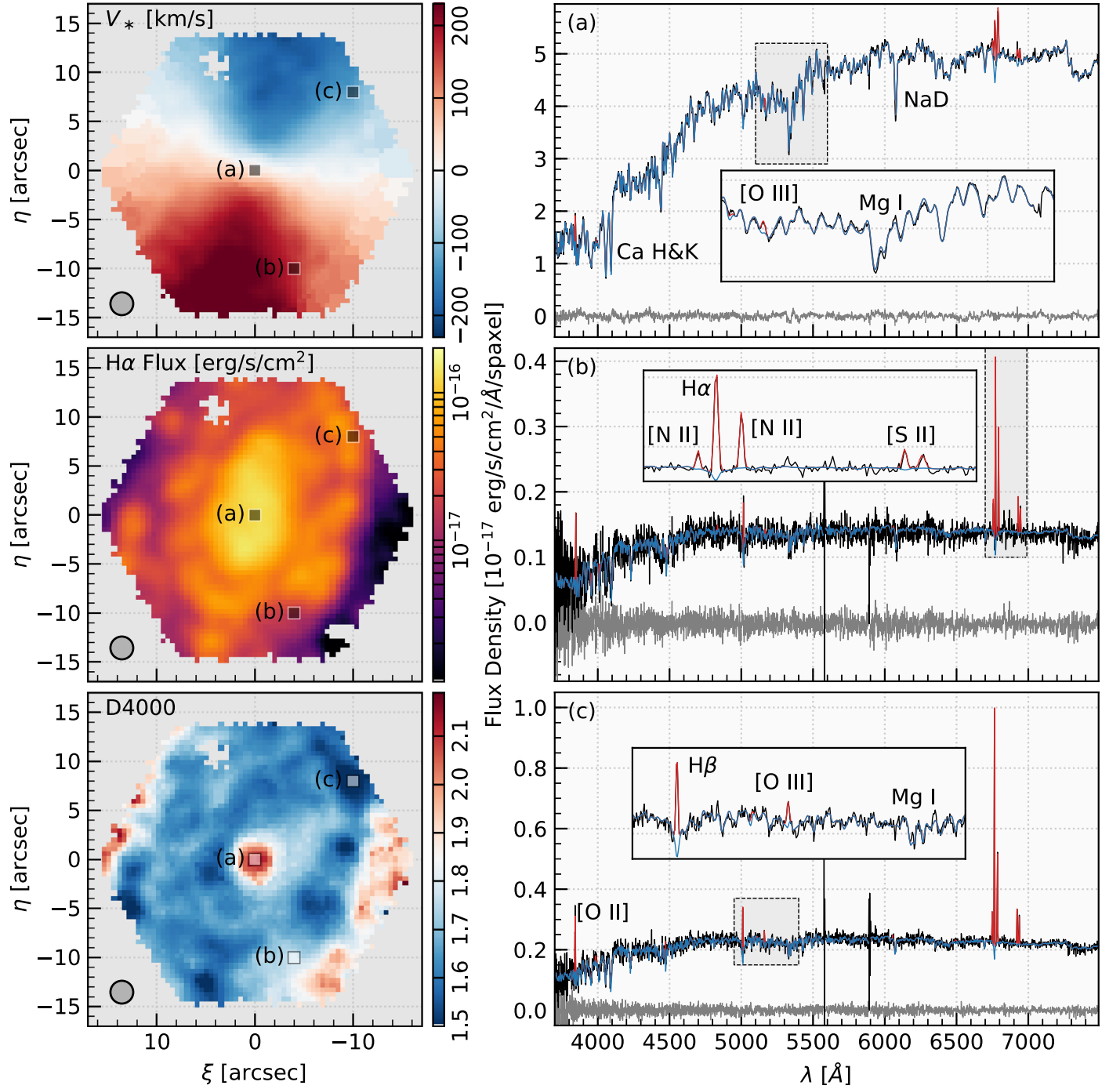
Figure 4. Example data provided by the MaNGA data analysis pipeline (DAP) for MaNGA observation 8138-12704, MaNGA ID 1-339041, following the hybrid-binning approach (DAPTYPE is HYB10-GAU-MILES HC). The left column shows maps, or images, of some of the DAP-derived quantities, namely, from top to bottom, the stellar velocity field, H\alpha flux, and D4000 spectral index, where the measured value is indicated by the colorbar to the right of each map panel. The effective beam size for the MaNGA observations ( \text{FWHM} \sim 2''.5 ) is shown by the gray circle in the bottom left of each map panel. Three spaxels are highlighted and labeled (a), (b), and (c), according to their spectra plotted in the right column. Each spectrum panel shows the observed MaNGA spectrum (black), stellar-continuum-only model (blue), and best-fitting (stars+emission lines) model (red); the residuals between the data (black) and the model (red) are shown in gray. Note that the red and blue lines are identical except for regions with nebular emission. A few salient emission and absorption features are marked in each panel. Inset panels provide a more detailed view of the quality of the fitted models in the regions highlighted by gray boxes. The spectrum panels only show the spectral regions fit by the DAP, which is limited by the MILES spectral range for DR15.
