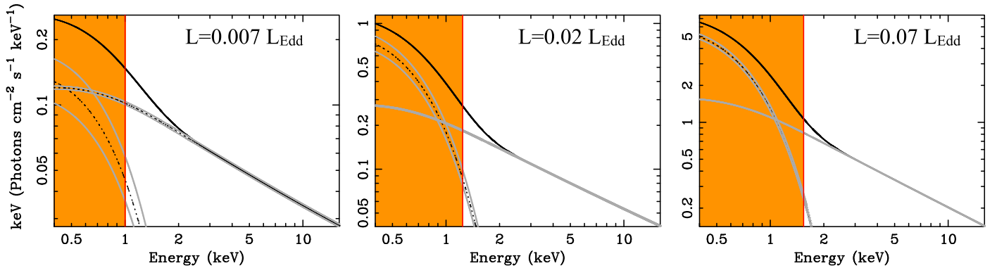
Figure 5. Best-fit models for the continuum of GX 339-4 (in the XMM-Newton data sets). The model used is tbabs * [ diskbb + nthcomp ], though in the plots the absorption component is removed. The shaded area marks the energies where the reverberation lag is observed in the high-frequency lag-energy spectra of Figure 2.
