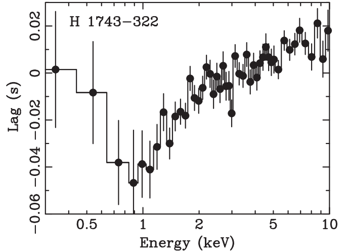
Figure 8. Lag-energy spectrum of H1743-322 in the frequency interval 0.1–1 Hz.
