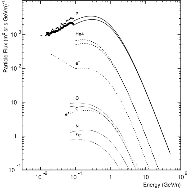
Fig. 2. Predictions of cosmic-ray energy spectra after the Solar Orbiter launch. The top and bottom continuous (protons) and dashed ( ^4\text{He} nuclei) curves are obtained with the G&A model above 70 MeV/n for minimum and maximum solar modulation parameter values of 300 MV/c and 340 MV/c, respectively. Maximum ( \phi=300 MV/c) and minimum ( \phi=340 MV/c) proton and helium predictions apply to years 2020 and 2022, respectively. The dot-dashed (dotted) curves indicate the electron and positron (nucleus) energy spectra at solar minimum.
