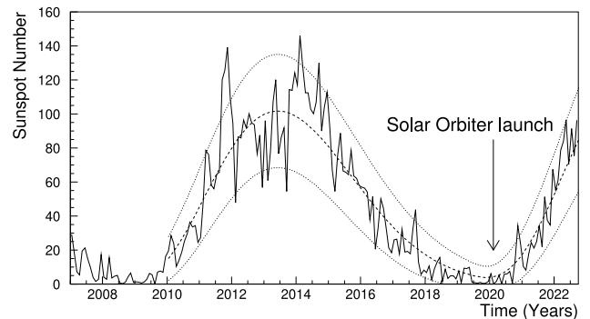
Fig. 1. Average monthly sunspot number observed since 2006 during solar cycles 24 and 25. Minimum and maximum predictions (top and bottom dotted lines) are gathered from http://solarcycle.science.com/solarcycle.html .
