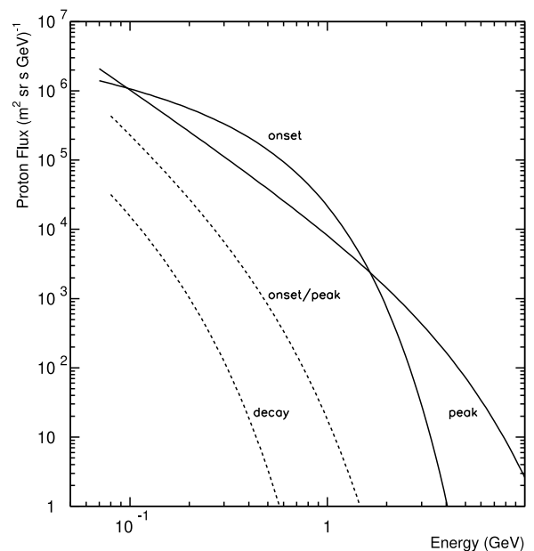
Fig. 3. Solar proton energy spectra measured by the PAMELA experiment during the evolution of the SEP events dated December 13 (solid lines) and December 14 (dashed lines), 2006. The different phases of the events are indicated in the figure.
