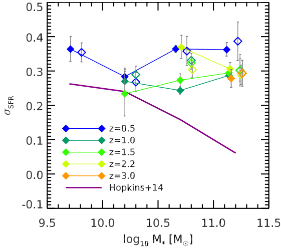
Fig. 12. Evolution of the \log_{10}(SFR) dispersion as a function of both redshift and stellar mass. Each color is showing a different redshift bin. Filled symbols show the result of scatter stacking, while open symbols show the dispersion estimated from individual Herschel detections above the main sequence (see text). The open symbols have been shifted up by 0.1 dex in mass for clarity. Errors are from bootstrapping in all cases. We compare these to the typical scatter of the SFHs in the numerical simulation of Hopkins et al. (2014) shown as a solid purple line.
