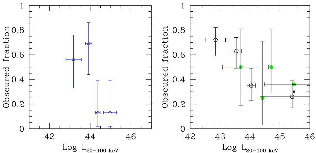
Figure 6. Fraction of obscured AGN (number of objects with N_H > 10^{22} \text{ cm}^{-2} over the total number) versus luminosity bins, computed for the 64 hard X-ray selected radio galaxies (left-hand panel). Fraction of obscured AGN versus luminosity bins, computed for the Malizia et al. (2012) sample (right-hand panel). Non-radio galaxies are drawn as black open polygons, while radio galaxies as green filled polygons.
