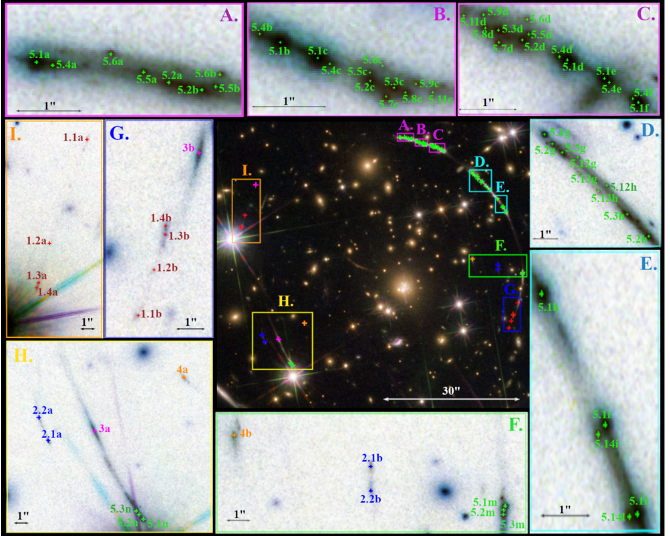
Fig. 1. HST color composite image of PSZ1-G311 with all cataloged multiple images shown. The first segment of the Sunburst Arc is highlighted in the magenta cut-outs A, B and C, and with the cyan cut-outs D and E, we can see almost all families of Sys-5, marked in green. Sys-1 (in red) is visible in both the orange (I) and blue (G) cut-out. In the latter we can also see family 3b, marked in magenta. Sys-2 (in blue) is visible in both the yellow (H) and green (F) cut-out. In cut-out H we can also see family 4a (in orange) and 3a, 5.1n, 5.2n, 5.3n. Images 4b, 5.1m, 5.2m, and 5.3m are visible in cut-out F.
