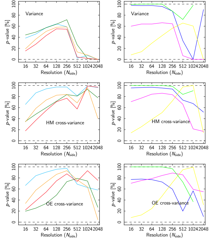
Fig. 6. Lower-tail probabilities of the variance determined from the Commander (red), NILC (orange), SEVEM (green), and SMICA (blue) component-separated polarization maps (left) and the SEVEM-070 (light green), SEVEM-100 (dark blue), SEVEM-143 (yellow), and SEVEM-217 (magenta) frequency-cleaned maps (right) at different resolutions. The top, middle and bottom rows correspond to results evaluated with the full-mission, HM- and OE-cross-variance estimates, respectively. In this figure, small p -values would correspond to anomalously low variance.
