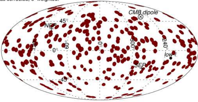
Fig. 32. Impact of bias correction and weighting on the uniformity of dipole directions for E -mode polarization HMHD simulation maps. Upper panel: local-variance dipole directions for the Commander simulations of E -mode polarization maps, obtained for 4^\circ discs, when no bias correction and weighting have been applied to the maps. Middle panel: same as in the upper panel, but when the transformation X_i \rightarrow (X_i - M_i)/\sigma_i has been applied to the polarization maps before applying the local-variance estimator. Lower panel: same as in the upper and middle panels, but when the transformation X_i \rightarrow (X_i - M_i)/\sigma_i^2 has been applied to the maps (i.e., with a square in the denominator). The results for the other component-separation methods are very similar to the ones presented here. For reference, we also show the CMB dipole direction, the north ecliptic pole (NEP), the south ecliptic pole (SEP), and the preferred dipolar modulation axis (labelled as “low- l ”) derived from the temperature data in Sect. 7.2.
