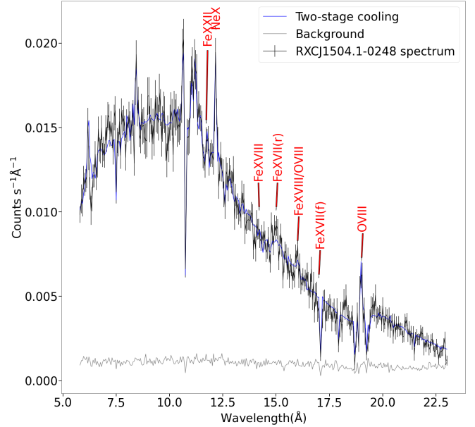
Figure 1. Stacked first order RGS spectrum of RXCJ1504.1-0248 in rest wavelength. The RGS spectrum is shown in black and the best fit two-stage cooling models is seen in blue. The background is seen in grey. Strong emission lines are labelled in red. The spectrum is overbinned by a factor of 6 for plotting purposes.
