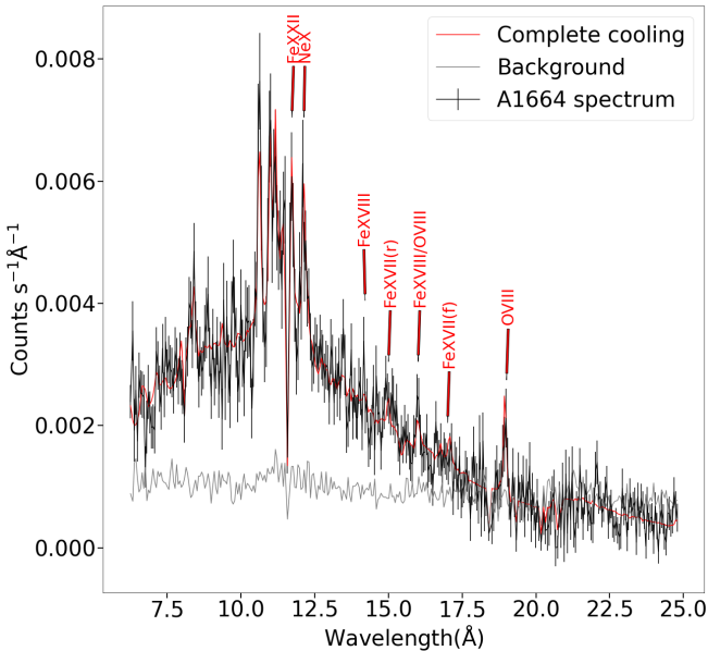
Figure 2. As Fig. 1, the stacked RGS spectrum of A1664 with the best fit complete cooling flow model in red in rest wavelength.
