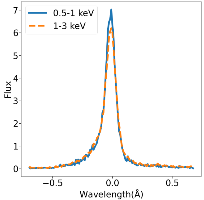
Figure 4. The energy dependent surface brightness profile of A1664.
