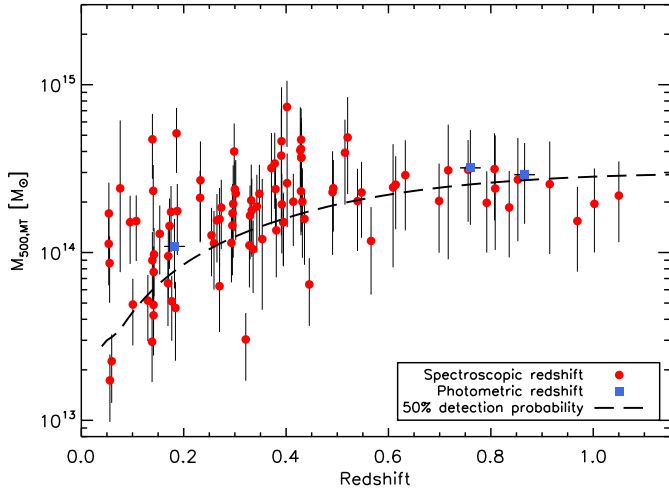
Fig. 6. Distribution of the bright XXL cluster sample in the M_{500,MT} vs. redshift plane. Although many low mass systems are detected at low redshift ( \sim 20\% of the sample with M_{500,MT} < \times 10^{14} M_{\odot} ), the high redshift subsample mostly contains similar mass clusters. The dashed line shows the 50% completeness limit in the WMAP9 cosmology from the model described in Sect. 6.1.
