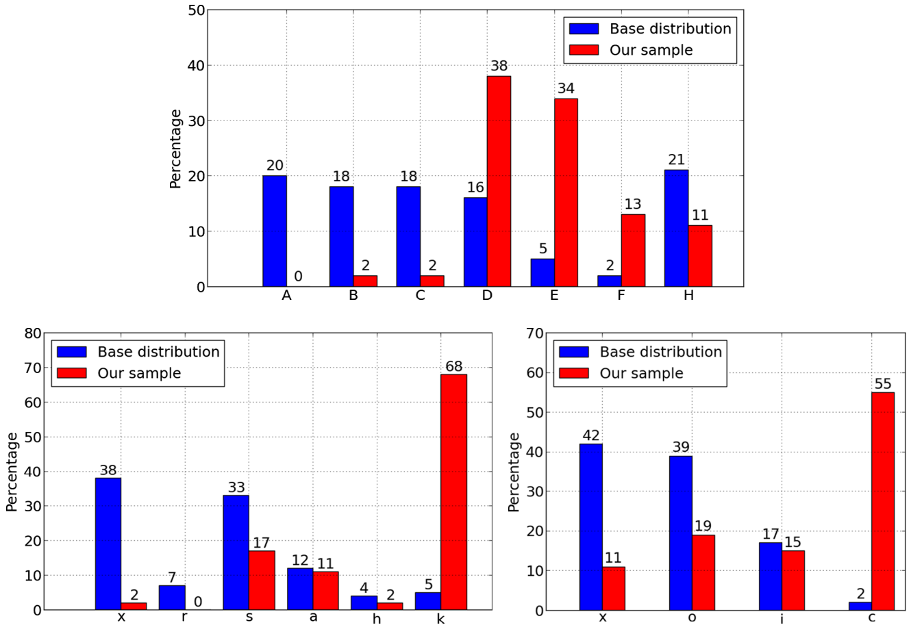
Fig. 4. Distribution of the McIntosh classes of the active regions associated with the selected CMEs. Top: Z code, bottom left: p code, bottom right: c code. The base distribution is that reported by McIntosh (1990) (calculated over the period 1969–1976).
