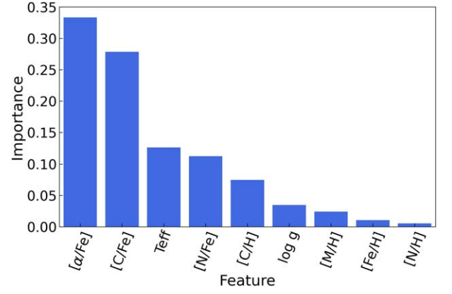
Figure 3. Stellar feature parameters extracted using the GBDT algorithm. The stellar features are sorted from left to right in order of importance, with the importance reflecting the contribution of that feature in the prediction model.
