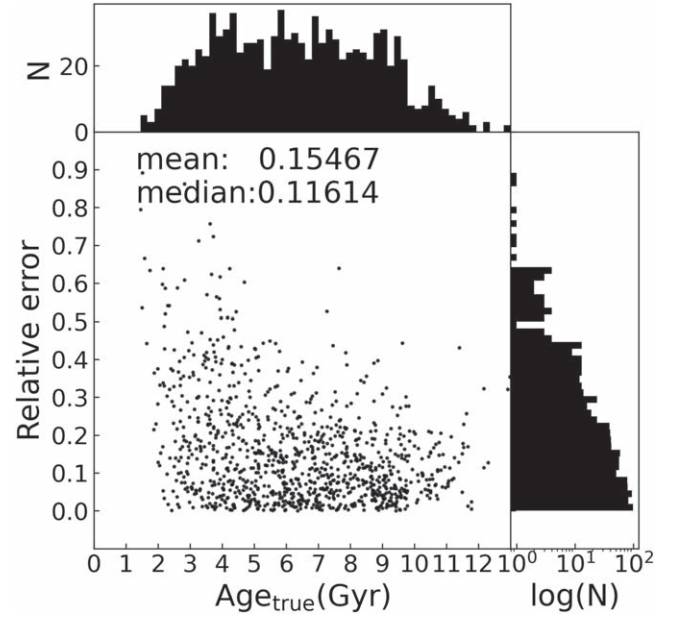
Figure 7. The mean and median relative error of predicted age for the test data set. The black dots represent the relative error in age, the top histogram is the star counts, and the right panel shows the distribution of the relative age error in terms of values. The relative error is the absolute error divided by the true values. It is naturally found that the errors should be small since they are from the same catalog but divided into testing and training.
