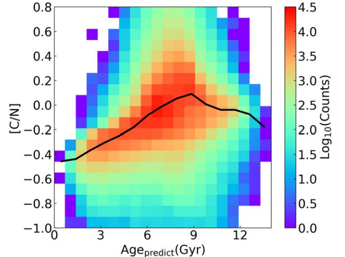
Figure 13. Relationship between the predicted age and the [C/N] ratio. The colors indicate the logarithmic values of the number of stars. The black line denotes the median value of the [C/N] ratio in each bin.
