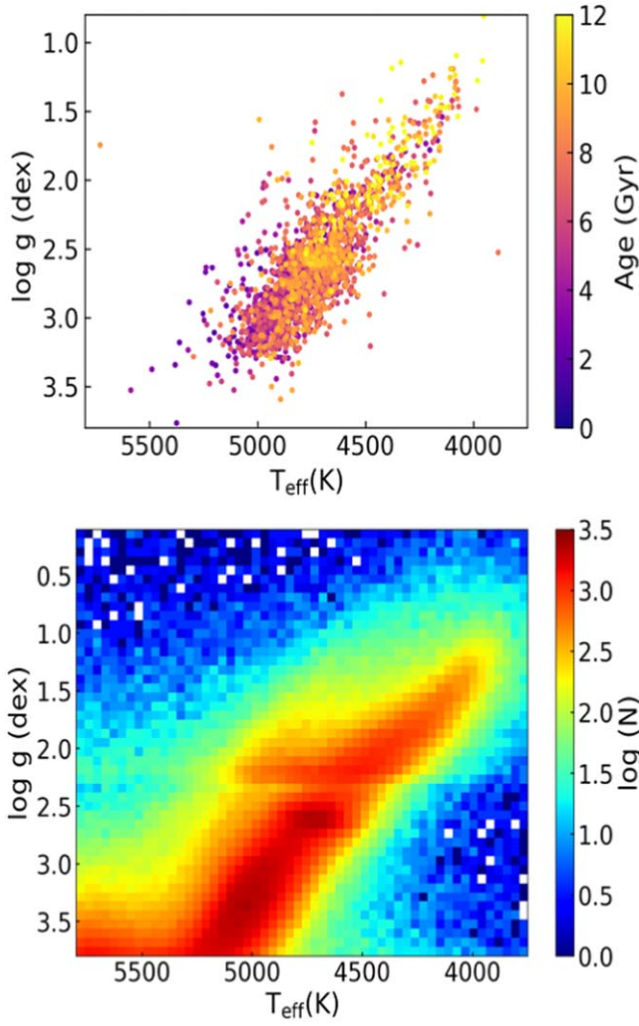
Figure 1. T_{\text{eff}}\text{--}\log g diagram of the sample used in this paper. The upper panel shows a Kiel diagram of the RGB stars selected from the APOKASC-2 catalog as the final small training sample, and the colors indicate the stellar ages. The lower panel shows a Kiel diagram of the large sample to be estimated using the GBDT method. The sample of RGB is identified by Wang et al. (2023c) from LAMOST DR8, with purity and completeness exceeding 95%.
