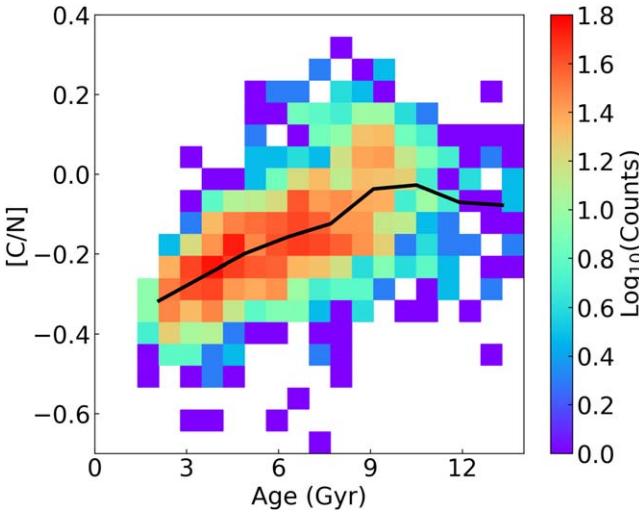
Figure 2. [\text{C}/\text{N}] –age diagram of the training sample used in this paper, with the color indicating the stellar density in the log scale showing that both parameters are correlated with each other.
