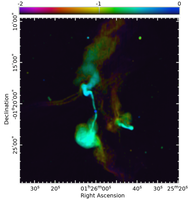
Fig. 18. Log intensity-coded MGCLS spectral index map of the 3C40A and 3C40B radio sources in Abell 194, at full resolution ( 7.7'' \times 7.5'' ). Colours indicate the spectral index, and the brightness indicates the Stokes- I intensity. The colour bar indicates the spectral indices, with the upper (lower) part of the colour bar corresponding to the brighter (fainter) regions. The brightness is on a linear scale and saturates at 8 \text{ mJy beam}^{-1} .
