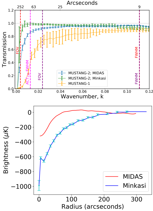
Figure 14. Top: the transfer function of MUSTANG-2 shows a marked improvement over that of MUSTANG-1. We also note the overlap with ACT (especially the band centered at 146 GHz, noted as 150 in this figure). Bottom: the surface brightness profile for Zwicky 3146 as determined by Minkasi (in concentric annuli, as plotted) and by MIDAS; the impact of the transfer function(s) is evident.
