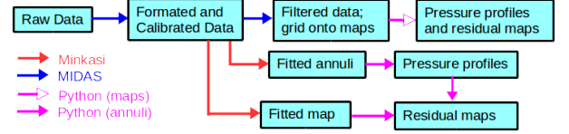
Figure 13. Flowchart for how various data products are produced.
