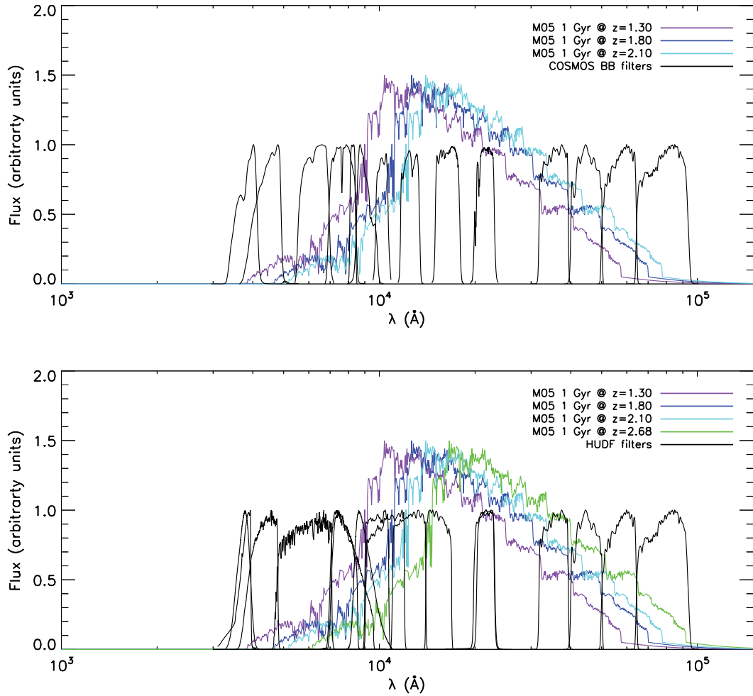
Figure 4. Top panel: as in Fig. 3, but now considering only filters matching in effective wavelength and bandpass the HUDF ones. All medium-band filters but one (SuprimeCam IA827 ) are discarded. Bottom panel: as in the top panel, but for filters available in the CANDELS HUDF catalogue. One additional M05 SSP at z = 2.68 is plotted to encompass the redshift range of the HUDF sample.
