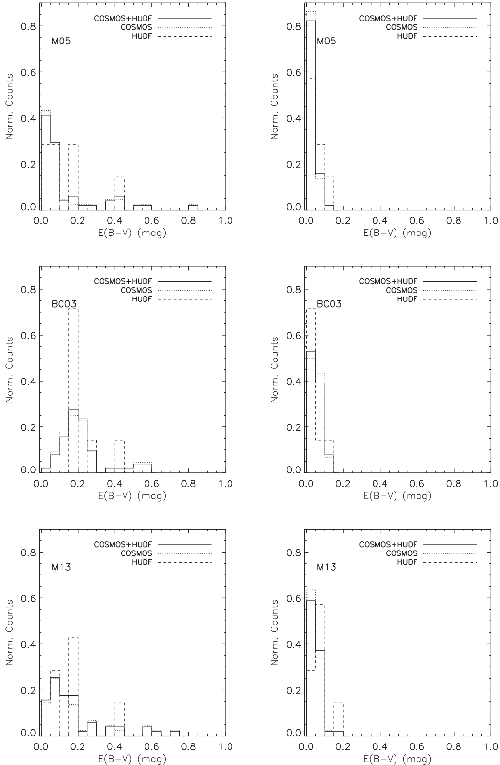
Figure 11. Normalized distributions of E(B - V) for HUDF, COSMOS and HUDF+COSMOS galaxies obtained with M05 , BC03 and M13 models (from top to bottom). Left-hand and right-hand panels refer to the samples prior and after discarding possible unreliable solutions according to Section 5.2.
