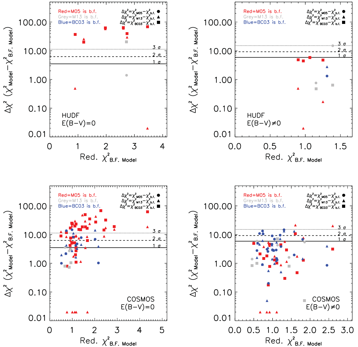
Figure 7. Significance of solutions around the best fit. For each galaxy, the lowest \chi^2_r value among those obtained using M05 , M13 and BC03 models is plotted on the x-axis. The \Delta\chi^2 between the best fit and the other solutions are plotted on the y-axis. Points are colour coded according to the model giving the lowest \chi^2_r value (red, grey and blue for M05 , M13 and BC03 , respectively) and different symbols are used to represent the models to which the differences refer to (dots for M05 , triangles for M13 , squares for BC03 ). Horizontal lines mark the 1\sigma , 2\sigma and 3\sigma confidence regions. Upper panels refer to the HUDF sample, lower ones to the COSMOS one. Left-hand and right-hand panels show the extinction-free and reddened cases. \Delta\chi^2 = 0 are plotted as \Delta\chi^2 = 0.02 for visibility reasons.
