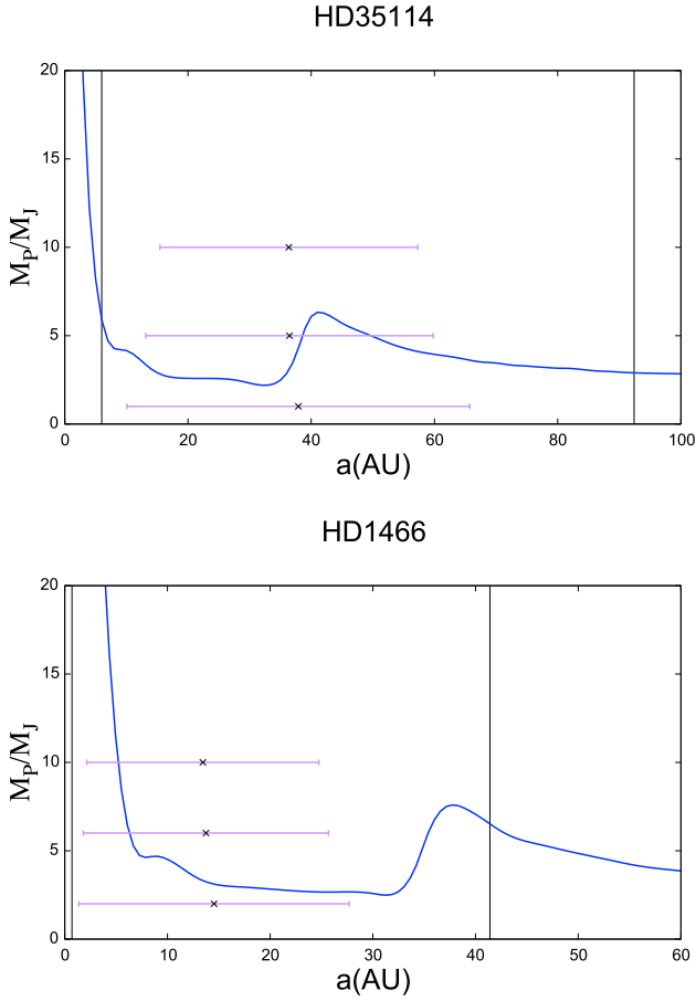
Fig. 4. SPHERE detection limits for HD 35114 (up) and HD 1466 (down). The bar plotted for each M_p represents the interval of distances covered by the planet during its orbit, from a minimum distance (periastron) to the maximum one (apoastron) from the star. The two vertical black lines represent the positions of the two belts. Projection effects in the case of significantly inclined systems are not included.
