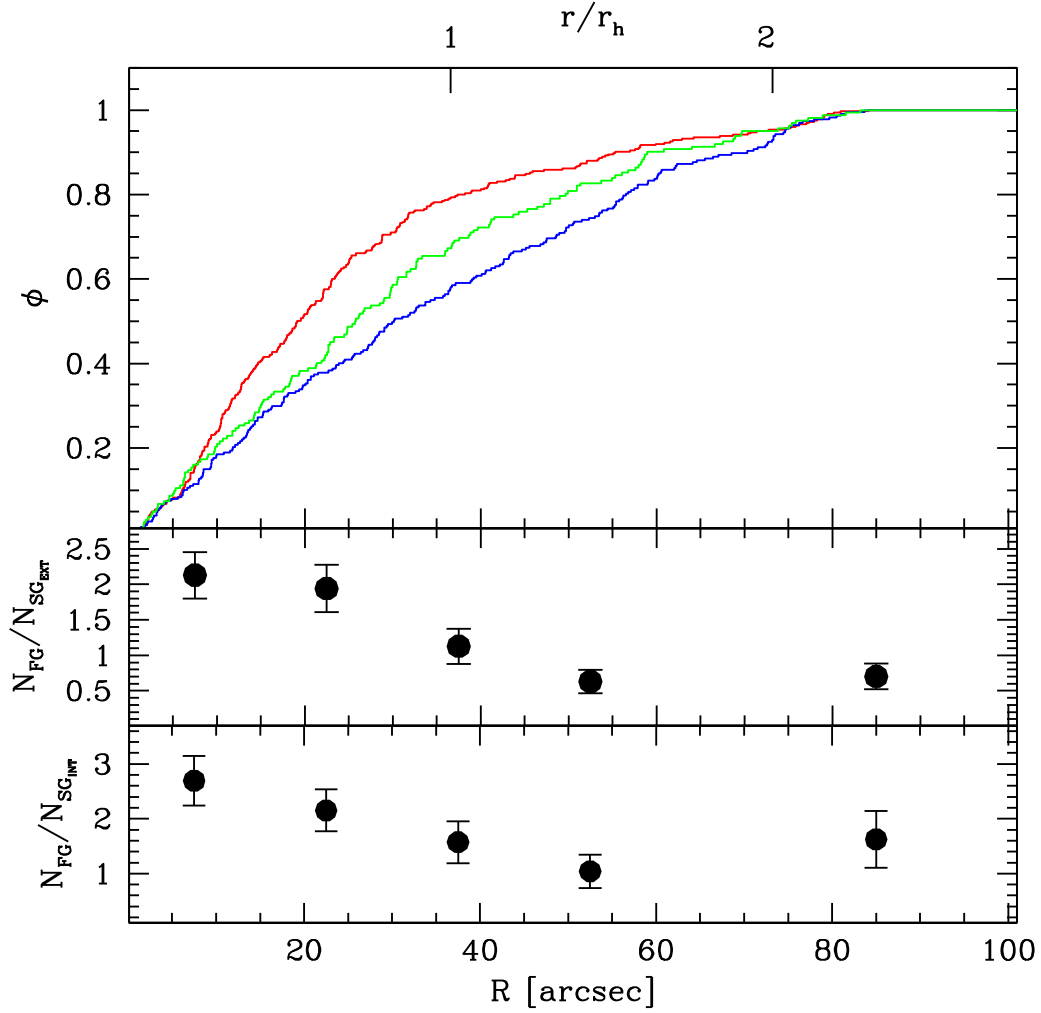
Figure 4. Upper panel: cumulative radial distribution of FG (red), SG INT (green), and SG EXT (blue) stars selected as detailed in Section 3. Lower panels: N_{\text{FG}}/N_{\text{SGINT}} and N_{\text{FG}}/N_{\text{SGEXT}} as a function of the distance from the cluster center.
