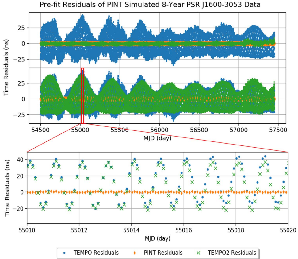
Figure 8. The residual difference due to different precession–nutation models. We use PINT to simulate 8 yr regularly sampled (2.4 hr cadence) TOAs with a simple timing model, only has a constant pulse frequency, and pulsar position. Orange marks represent the PINT residuals, the blue points are the TEMPO residuals, and green data points mark the TEMPO2 residuals. The first panel on the top shows the PINT and TEMPO/TEMPO2 residuals when TEMPO2 is under the IAU 2000 resolution of precession and nutation. The second panel displays the same results with TEMPO2’s old precession and nutation mode, and TEMPO2’s residuals have a similar signature to TEMPO residuals. The third panel is a zoomed-in version of the second panel on days from MJD 55010 to MJD 55020. We can see the diurnal sinusoidal oscillation from the TEMPO/TEMPO2 residuals. Given the sampling rate of NANOGrav 11 yr data, the TEMPO prefit residual differences in Figure 7 is one trace of the blue dots.
