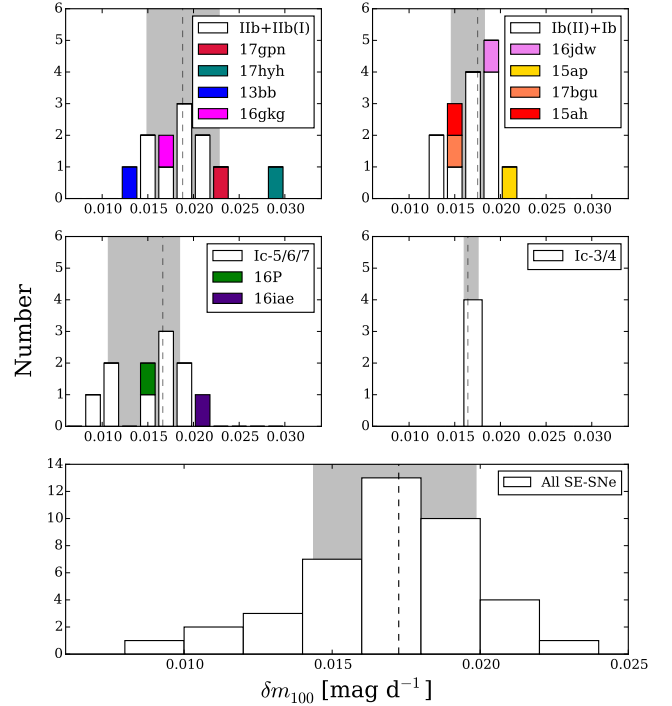
Figure 12. (top) The distribution of late time decay rates for SE-SNe; the median is \sim 0.017 \text{ mag d}^{-1} for all SN types. Only SN 2013bb has had host-galaxy flux subtracted, but the effect of this on \delta m_{100} was found to be negligible at this phase, \sim 0.001 \text{ mag d}^{-1} . The dashed line and grey regions are as in Figure 9.
