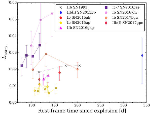
Figure 8. The normalised luminosity of the [O I] \lambda\lambda 6300,6363 line as derived from the nebular and near nebular spectra. Shown for reference is L_{\text{norm}} of type I Ib SN 1993J (Barbon et al. 1995; Richmond et al. 1996).
