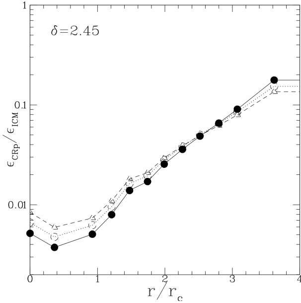
Figure 4. Upper limits to the ratio of the CRp to the thermal ICM energy densities as a function of radius. The three models assumes \eta_B = 0 (dashed), 0.3 (dotted) and 0.5 (solid) and the corresponding values of the lower-limit to the central magnetic fields B_0 from Figure 3 (left).
