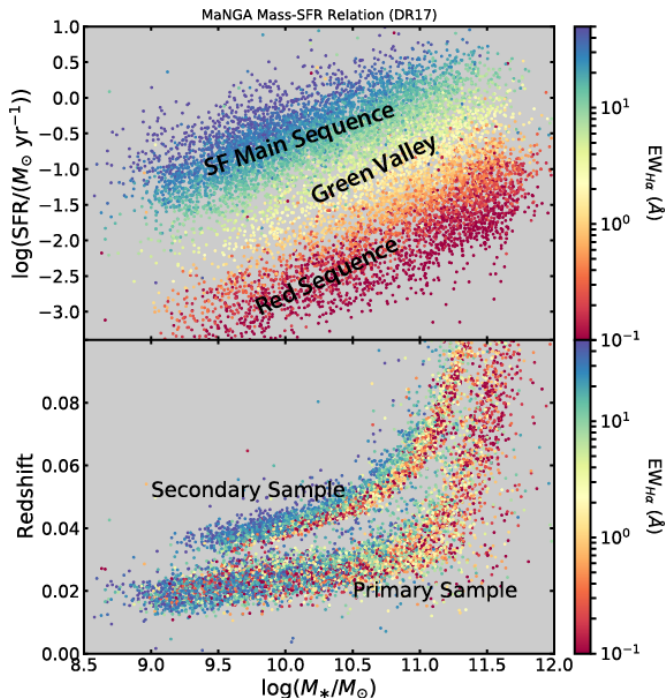
Figure 1. Stellar mass vs redshift and total H\alpha -derived SFR (uncorrected for dust extinction) within the IFU field of view for the MaNGA MPL-11 galaxy sample. Each point represents one of the \sim 10,000 galaxies in MPL-11, and are color coded by their integrated H\alpha equivalent width. The Primary ( 1.5R_e ) and Secondary ( 2.5R_e ) samples define a clearly offset trend in redshift at fixed stellar mass.
