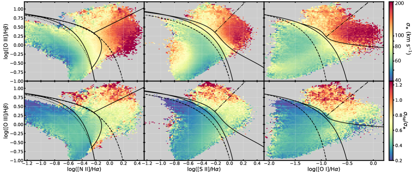
Figure 4. As Figure 2, but showing pixels color-coded by the median stellar velocity dispersion, and the median ratio between gas-phase and stellar velocity dispersion. Note the strong evolution of the relative velocity dispersions, in which the ionized gas dispersions are significantly smaller than the stellar dispersion in the star-forming region, only slightly smaller than the stellar dispersions in the LI(N)ER region, and comparable to or in excess of the stellar dispersions in the AGN region.
