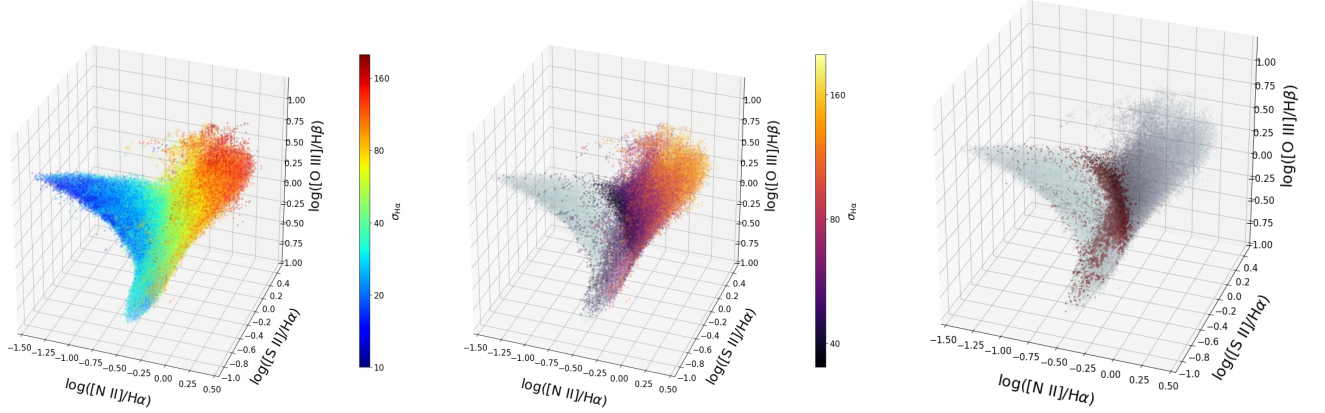
Figure 12. Left: 3D BPT diagram viewed at an elevation angle of 30^\circ . Data are binned in the 3D line-ratio space, and the bins are colored coded according to their sigma-clipped mean \sigma_{H\alpha} values. While a total of 75 \times 75 \times 75 bins are constructed, only bins made up of a minimum number of 5 spaxels are shown. An animated element shows the diagram rotating through different viewing angles. Middle: bins with \sigma_{H\alpha} < 35 \text{ km s}^{-1} are made transparent and only bins with \sigma_{H\alpha} > 35 \text{ km s}^{-1} are colored coded. Right: bins with \sigma_{H\alpha} = 33 - 37 \text{ km s}^{-1} are shown in red, of which the displayed sizes are set to be proportional to the number of spaxels inside the bins. The rest of the bins are made transparent.
