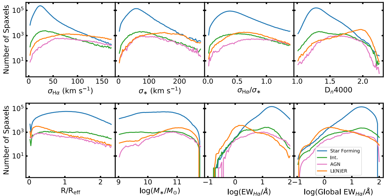
Figure 6. Histograms of galaxy properties in each of the four classes (star-forming, intermediate, AGN, and LI(N)ER) in the [\text{S II}]/\text{H}\alpha diagnostic diagram defined by Figure 2. Individual panels show distributions both in the properties of individual spaxels and in the overall galaxy-integrated stellar mass and global equivalent width of the host galaxies within which individual spaxels reside. Histograms for total galaxy mass and equivalent width have been lightly smoothed by a Savitzky-Golay filter to minimize high-frequency artifacts from the discrete integrated values across multiple spaxels.
