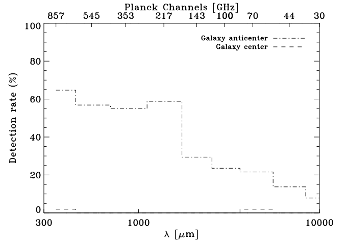
Fig. 6. Expected Planck capability of detecting the sample of UCHII analyzed here. Dashed line : true source Galactic position. Dot dashed line : results for the same population but located in the anticenter region.
