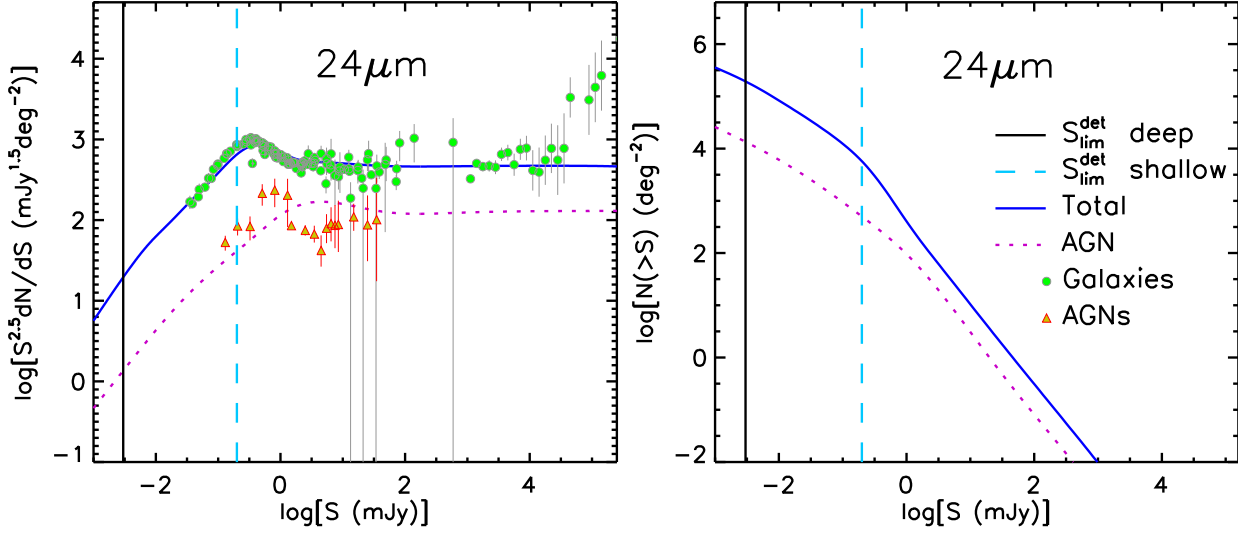
Figure 1. Euclidean normalized differential number counts (on the left) and integral counts (on the right) at 24\mu\text{m} given by the adopted model for galaxies as a whole (starburst plus AGN components; solid blue lines) and for AGNs alone (dotted violet lines). The vertical solid black and dashed cyan lines correspond to the SMI camera detection limits for the proposed deep and shallow surveys, respectively. Counts of galaxies (filled green circles) are from Takagi et al. (2012), Clements et al. (2011), Béthermin et al. (2010), Le Floc’h et al. (2009), Shupe et al. (2008), Papovich et al. (2004) and Sanders et al. (2003). The latter data show an excess at the highest flux densities due to the enhanced number of bright galaxies in the Virgo supercluster. AGN counts (red triangles) are from Treister et al. (2006) and Brown et al. (2006).
