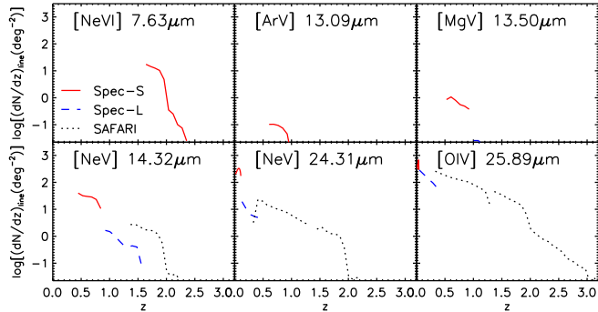
Figure 13. Predicted redshift distributions of AGNs detected in 6 lines ([NeVI]7.63, [ArV]13.09, [MgV]13.50, [NeV]14.32, [NeV]24.31 and [OIV]25.89 \mu\text{m} ) detected by SMI Spec-S (solid red lines) and Spec-L (dashed blue lines), compared, for three of them ([NeV]14.32, [NeV]24.31 and [OIV]25.89 \mu\text{m} ), with those obtained in Bonato et al. (2014b) for SPICA/SAFARI (dotted black lines), for an 1 h exposure per FoV.
