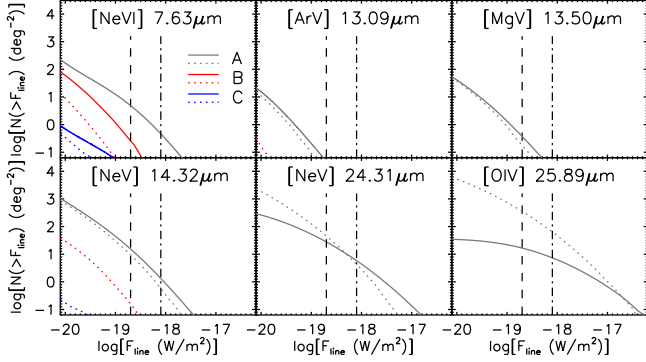
Figure 12. Contributions of different AGN populations to the SMI Spec-S (solid lines) and Spec-L (dotted lines) integral counts in 6 AGN lines ([NeVI]7.63, [ArV]13.09, [MgV]13.50, [NeV]14.32, [NeV]24.31 and [OIV]25.89 \mu\text{m} ). A: AGNs associated to late-type galaxies plus optically selected AGNs; B: AGNs associated to unlensed proto-spheroids; C: AGNs associated to strongly gravitationally lensed proto-spheroids. The vertical lines correspond to the detection limits ( 2.0 \cdot 10^{-19} \text{ W/m}^2 for Spec-S and 8.0 \cdot 10^{-19} \text{ W/m}^2 for Spec-L) for 1-h exposure per FoV.
