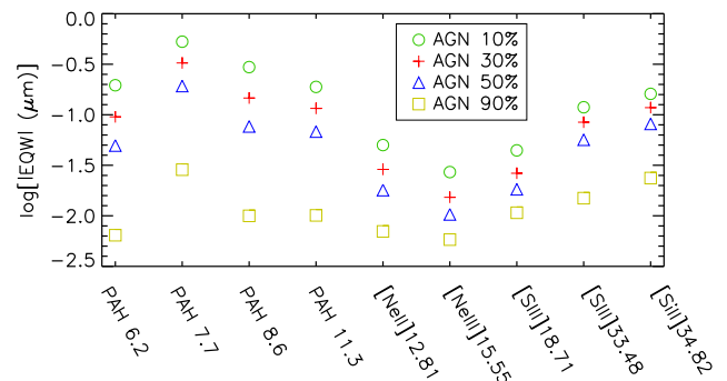
Figure 16. Equivalent widths (EQWs) of the brightest spectral lines in our sample for a galaxy with a fixed total (star forming plus AGN) IR luminosity of 10^{13} L_{\odot} and varying fractions of AGN IR luminosity.
