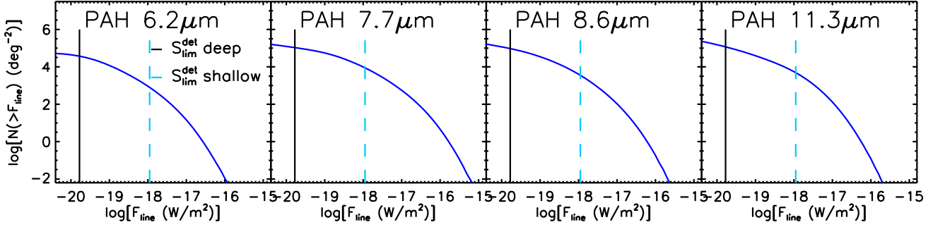
Figure 3. Integral counts in 4 PAH lines of star-forming galaxies over the SMI wide field camera wavelength range. The solid black and the dashed cyan vertical lines correspond to the SMI camera detection limits for the proposed deep and shallow surveys, respectively.
