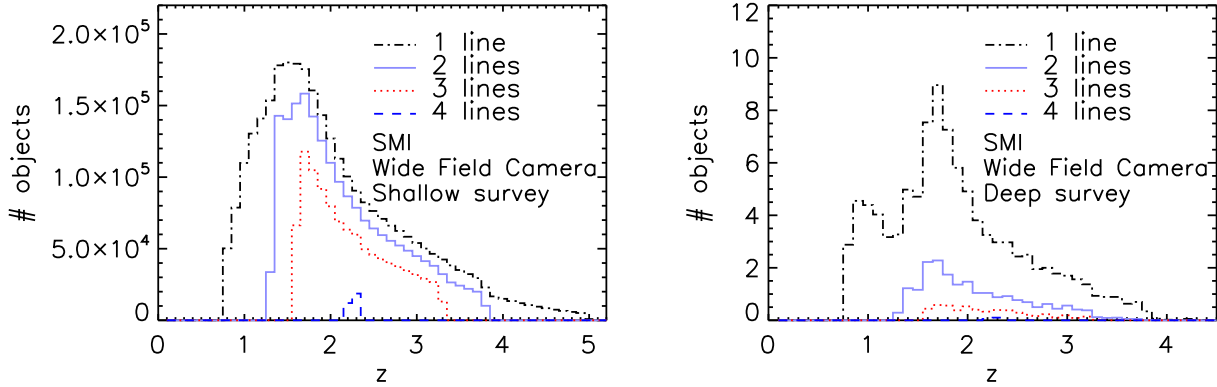
Figure 4. Redshift distributions of galaxies detected in at least 1 to 4 PAH lines by the proposed shallow (left panel) and deep (right panel) survey with the SMI wide-field camera.
