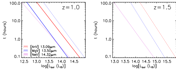
Figure 17. SPICA SMI Spec-S (solid lines) and Spec-L (dotted lines) exposure time per FoV required for a 5\sigma line detection of 3 typical AGN lines ([ArV]13.09, [MgV]13.50 and [NeV]14.32 \mu m) as a function of the AGN bolometric luminosity for z = 1.0 (left) and z = 1.5 (right).
