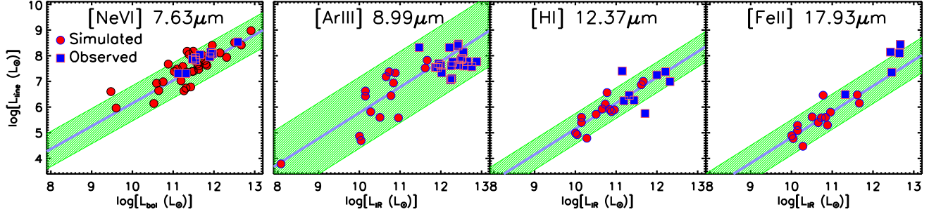
Figure 6. Comparison between observed (blue squares) and expected (red circles) line luminosities, obtained using ITERA (see Section 4 for details). The [NeVI]7.63 \mu\text{m} data (for AGNs) comes from the Sturm et al. (2002) and Veilleux et al. (2009) catalogues. For the other 3 lines the observed line luminosities (for star-forming galaxies) are from Willett et al. (2011). The green bands show the \pm 2\sigma dispersion around the line to continuum luminosity relations derived with ITERA.
